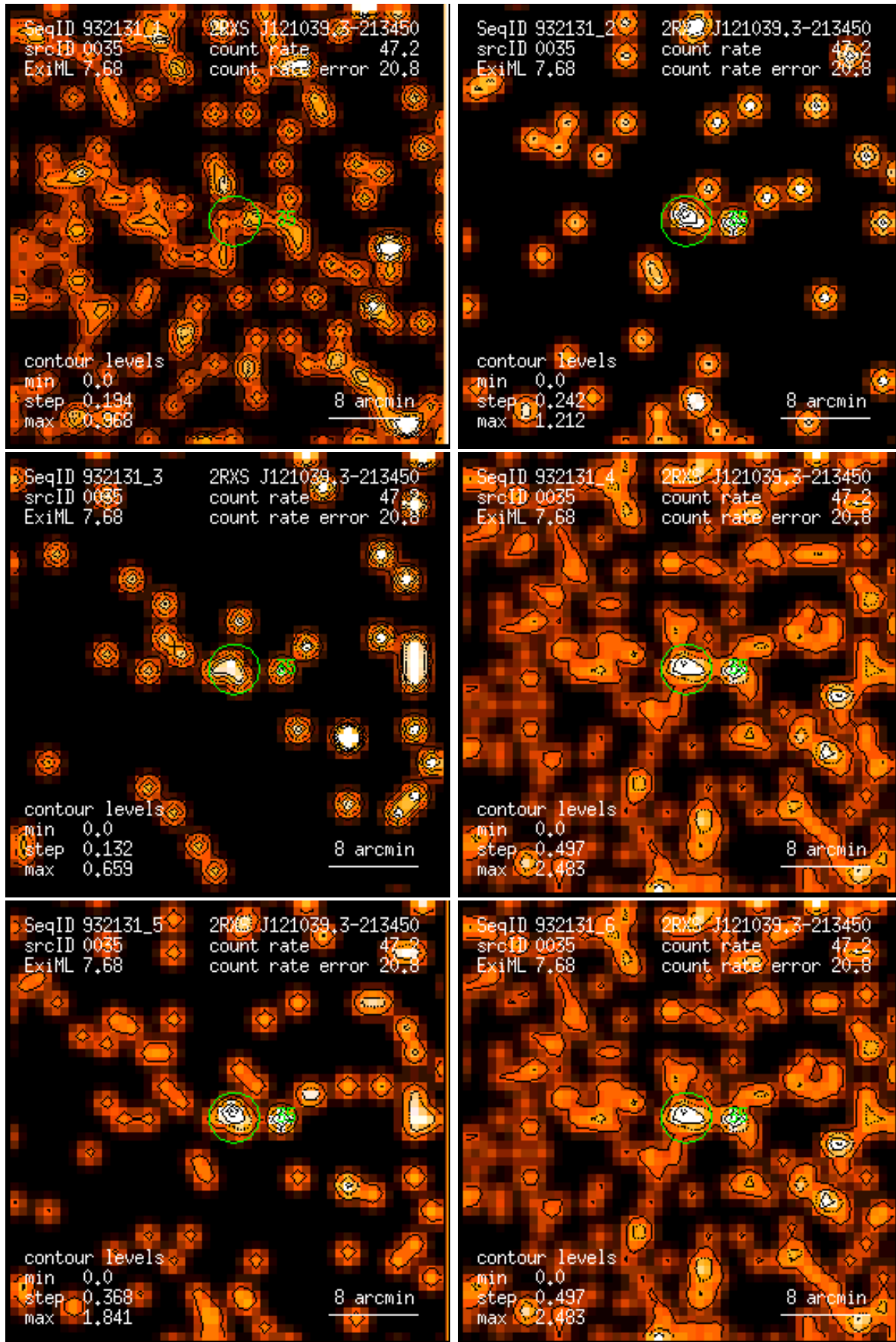
Figure 35: RASS 932131: detection 0035: band rate images, Gaussian filter: (1) PSPC channels 11 – 41, (2) 52 – 90, (3) 91 – 201, (4) 11 – 235, (5) 52 – 201, (6) 11 – 201. Broad band rates in counts/ks. Band rate contour levels in counts/ks/arcmin 2 .
