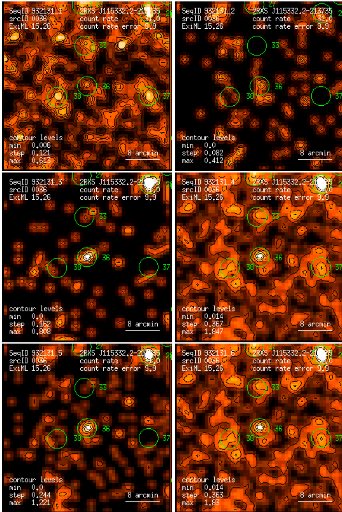
Figure 36: RASS 932131: detection 0036: band rate images, Gaussian filter: (1) PSPC channels 11 – 41, (2) 52 – 90, (3) 91 – 201, (4) 11 – 235, (5) 52 – 201, (6) 11 – 201. Broad band rates in counts/ks. Band rate contour levels in counts/ks/arcmin 2 .
