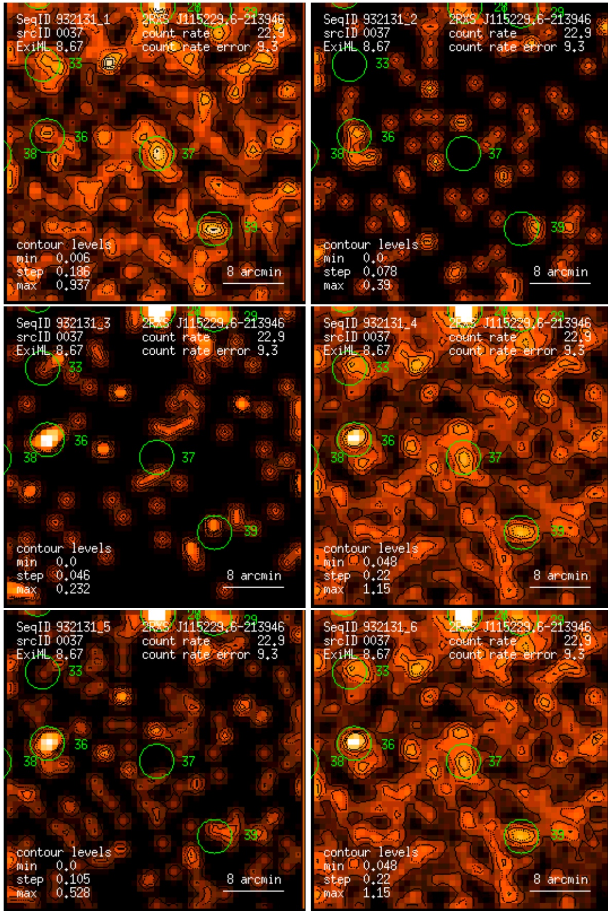
Figure 37: RASS 932131: detection 0037: band rate images, Gaussian filter: (1) PSPC channels 11 – 41, (2) 52 – 90, (3) 91 – 201, (4) 11 – 235, (5) 52 – 201, (6) 11 – 201. Broad band rates in counts/ks. Band rate contour levels in counts/ks/arcmin 2 .
