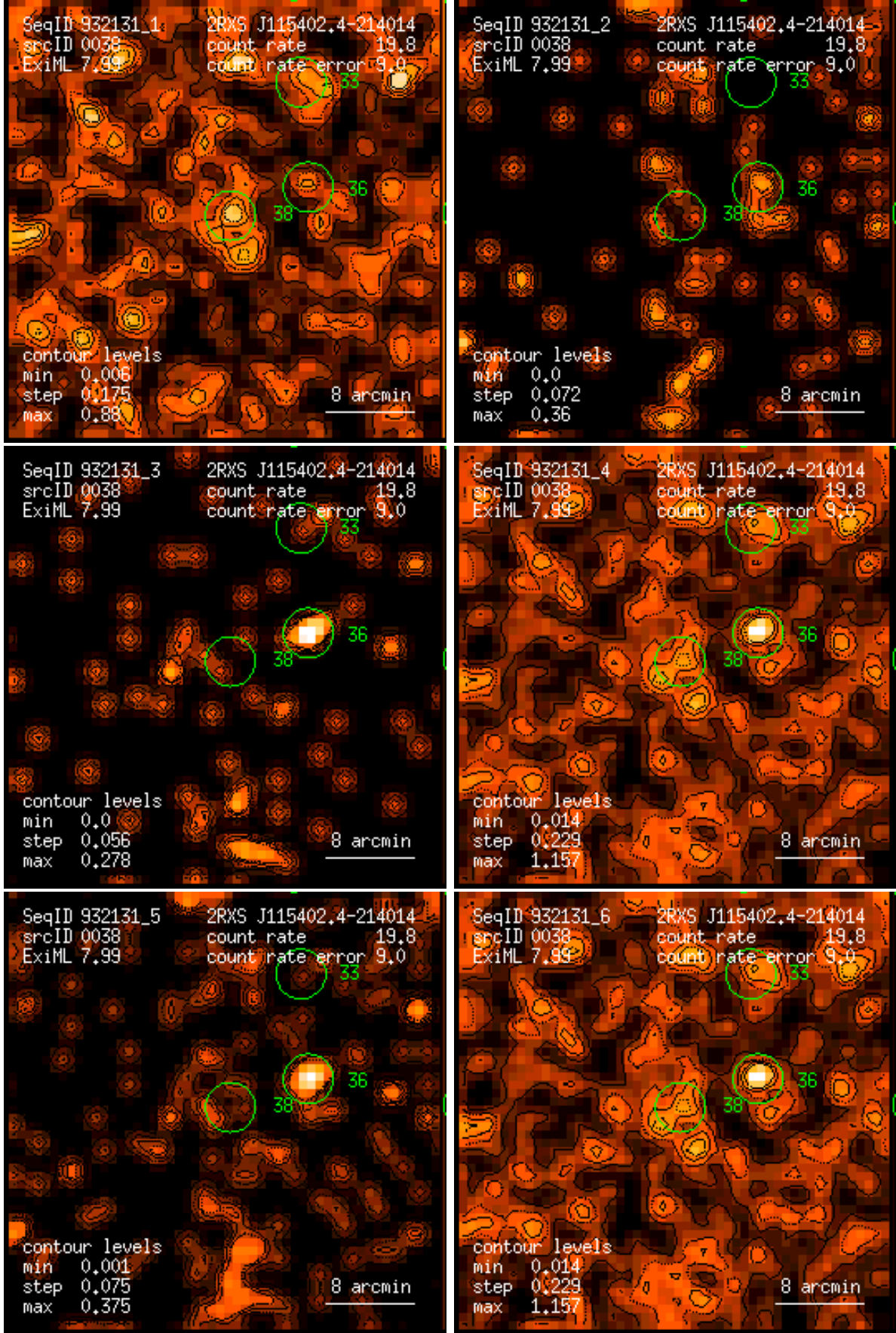
Figure 38: RASS 932131: detection 0038: band rate images, Gaussian filter: (1) PSPC channels 11 – 41, (2) 52 – 90, (3) 91 – 201, (4) 11 – 235, (5) 52 – 201, (6) 11 – 201. Broad band rates in counts/ks. Band rate contour levels in counts/ks/arcmin 2 .
