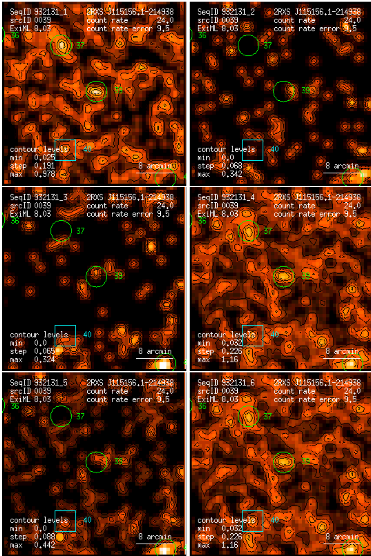
Figure 39: RASS 932131: detection 0039: band rate images, Gaussian filter: (1) PSPC channels 11 – 41, (2) 52 – 90, (3) 91 – 201, (4) 11 – 235, (5) 52 – 201, (6) 11 – 201. Broad band rates in counts/ks. Band rate contour levels in counts/ks/arcmin 2 .
