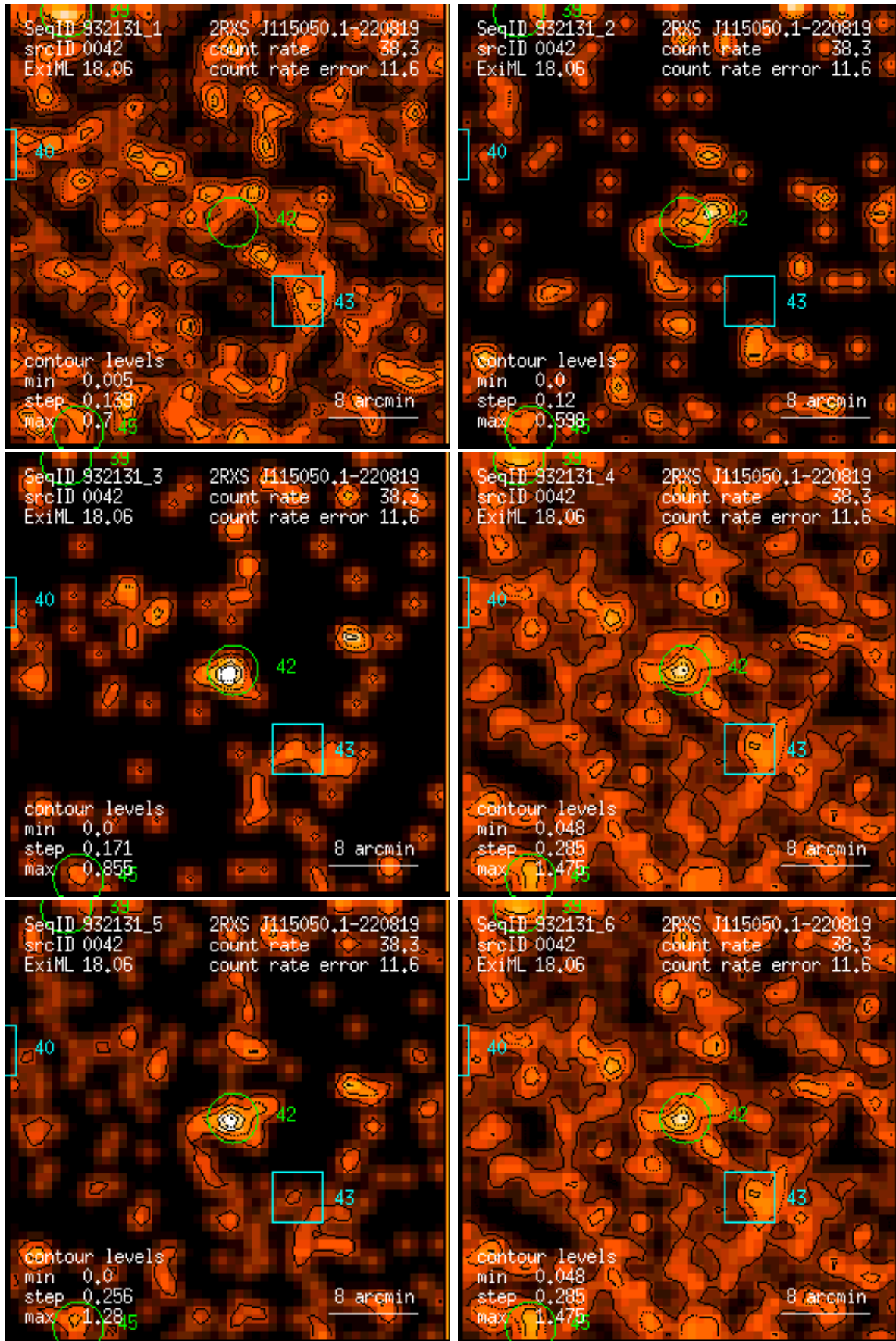
Figure 42: RASS 932131: detection 0042: band rate images, Gaussian filter: (1) PSPC channels 11 – 41, (2) 52 – 90, (3) 91 – 201, (4) 11 – 235, (5) 52 – 201, (6) 11 – 201. Broad band rates in counts/ks. Band rate contour levels in counts/ks/arcmin 2 .
