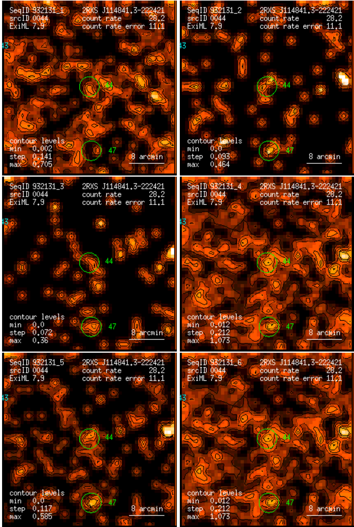
Figure 44: RASS 932131: detection 0044: band rate images, Gaussian filter: (1) PSPC channels 11 – 41, (2) 52 – 90, (3) 91 – 201, (4) 11 – 235, (5) 52 – 201, (6) 11 – 201. Broad band rates in counts/ks. Band rate contour levels in counts/ks/arcmin 2 .
