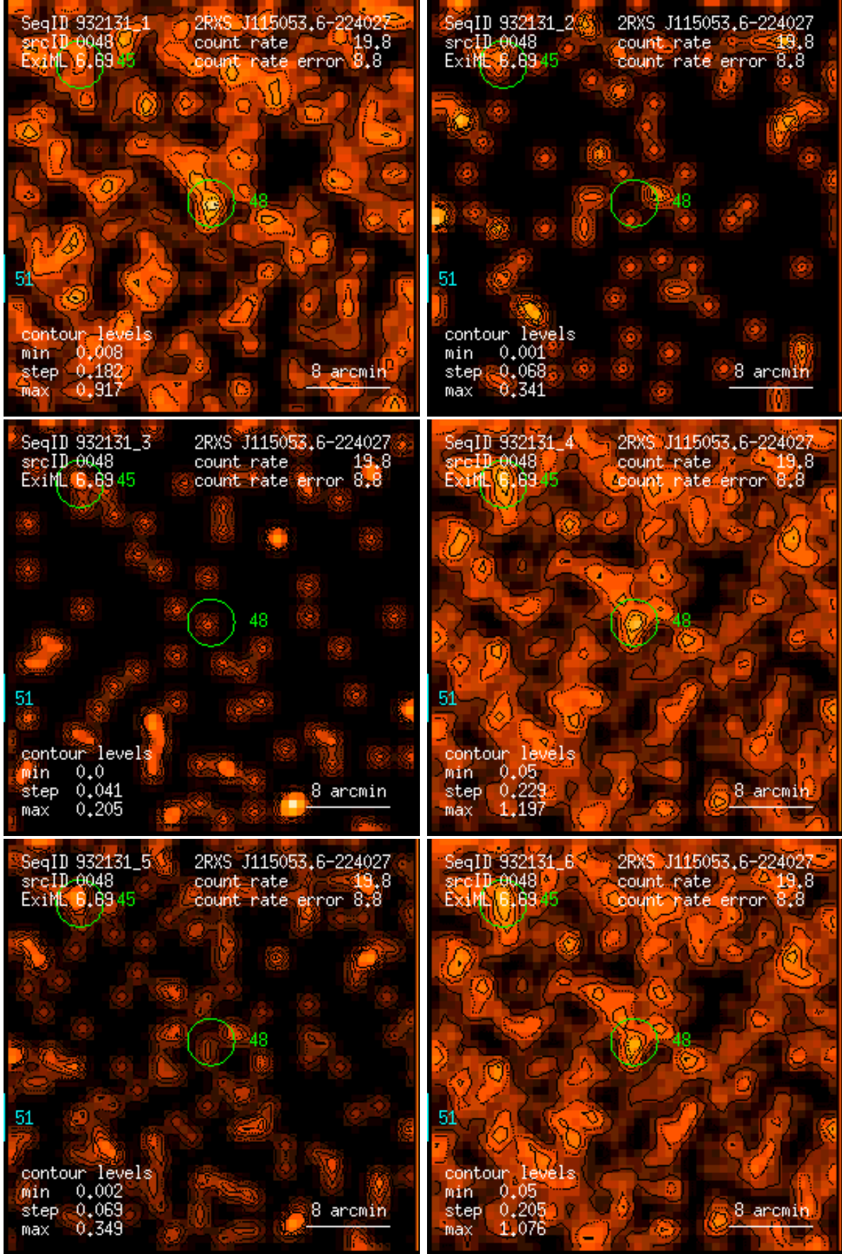
Figure 48: RASS 932131: detection 0048: band rate images, Gaussian filter: (1) PSPC channels 11 – 41, (2) 52 – 90, (3) 91 – 201, (4) 11 – 235, (5) 52 – 201, (6) 11 – 201. Broad band rates in counts/ks. Band rate contour levels in counts/ks/arcmin 2 .
