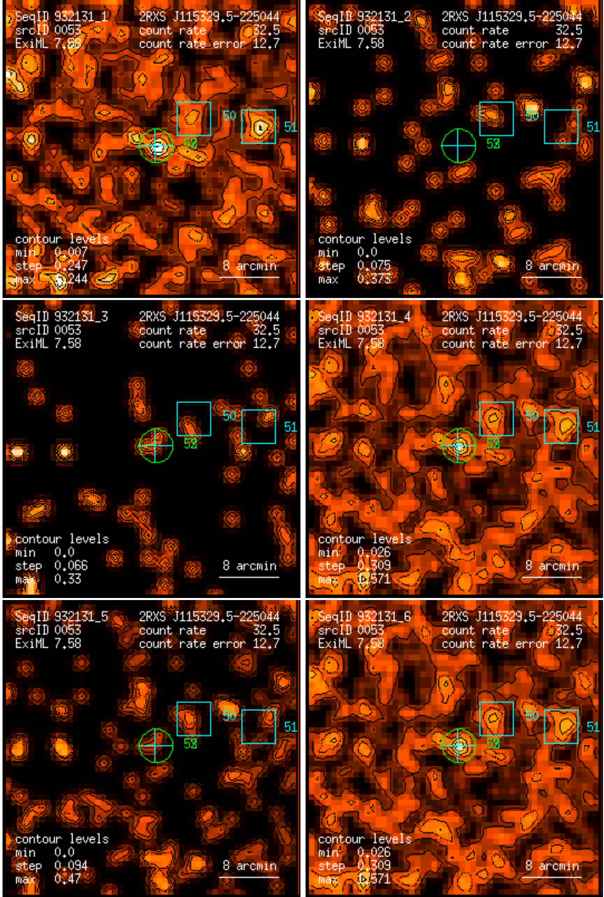
Figure 53: RASS 932131: detection 0053: band rate images, Gaussian filter: (1) PSPC channels 11 – 41, (2) 52 – 90, (3) 91 – 201, (4) 11 – 235, (5) 52 – 201, (6) 11 – 201. Broad band rates in counts/ks. Band rate contour levels in counts/ks/arcmin 2 .
