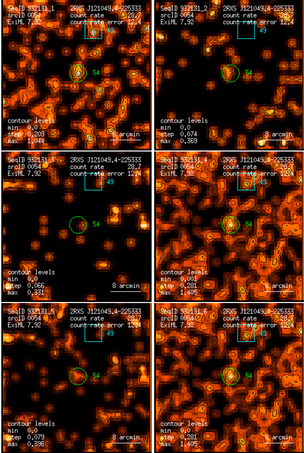
Figure 54: RASS 932131: detection 0054: band rate images, Gaussian filter: (1) PSPC channels 11 – 41, (2) 52 – 90, (3) 91 – 201, (4) 11 – 235, (5) 52 – 201, (6) 11 – 201. Broad band rates in counts/ks. Band rate contour levels in counts/ks/arcmin 2 .
