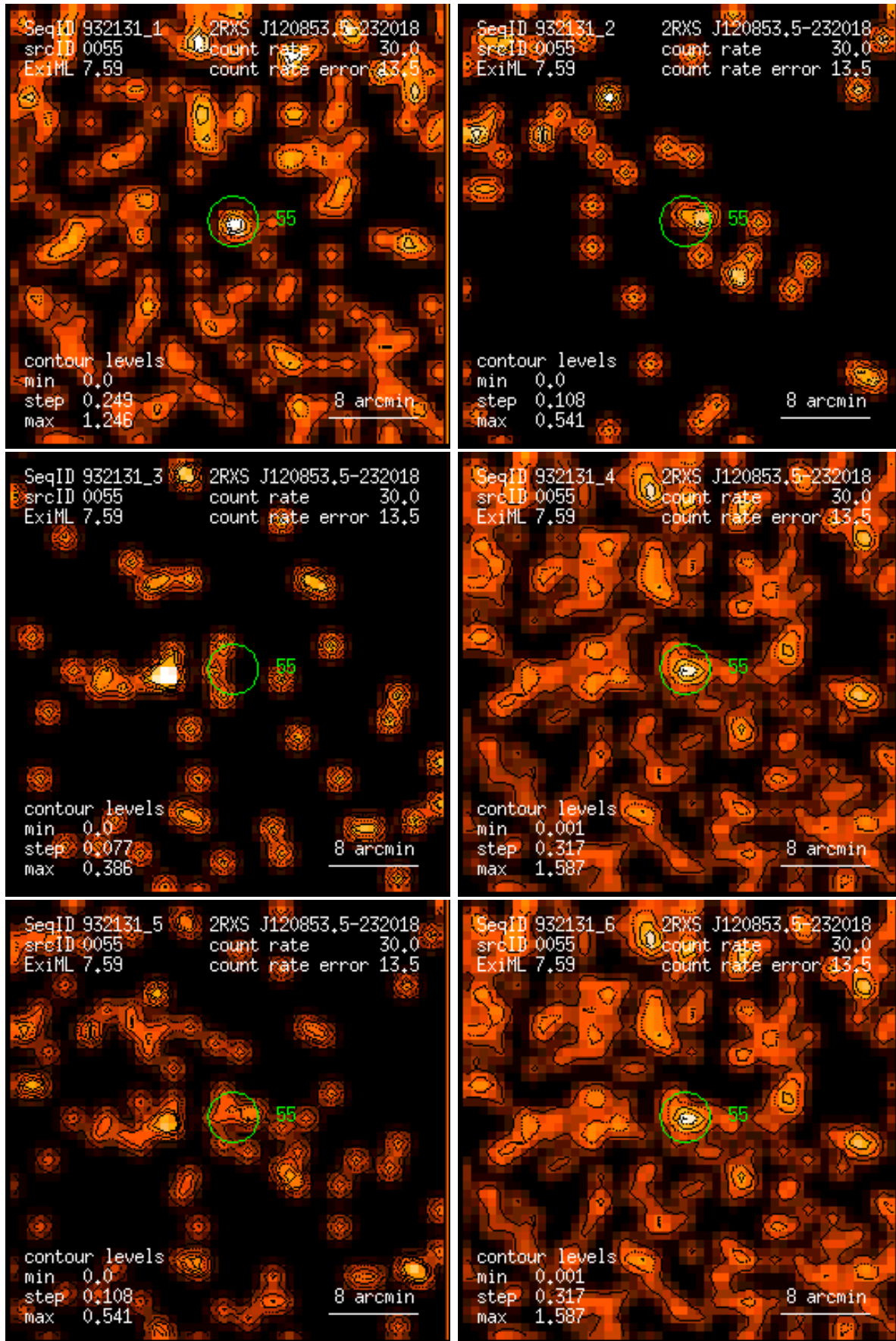
Figure 55: RASS 932131: detection 0055: band rate images, Gaussian filter: (1) PSPC channels 11 – 41, (2) 52 – 90, (3) 91 – 201, (4) 11 – 235, (5) 52 – 201, (6) 11 – 201. Broad band rates in counts/ks. Band rate contour levels in counts/ks/arcmin 2 .
