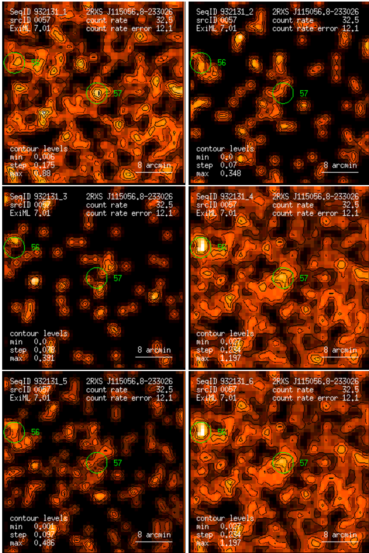
Figure 57: RASS 932131: detection 0057: band rate images, Gaussian filter: (1) PSPC channels 11 – 41, (2) 52 – 90, (3) 91 – 201, (4) 11 – 235, (5) 52 – 201, (6) 11 – 201. Broad band rates in counts/ks. Band rate contour levels in counts/ks/arcmin 2 .
