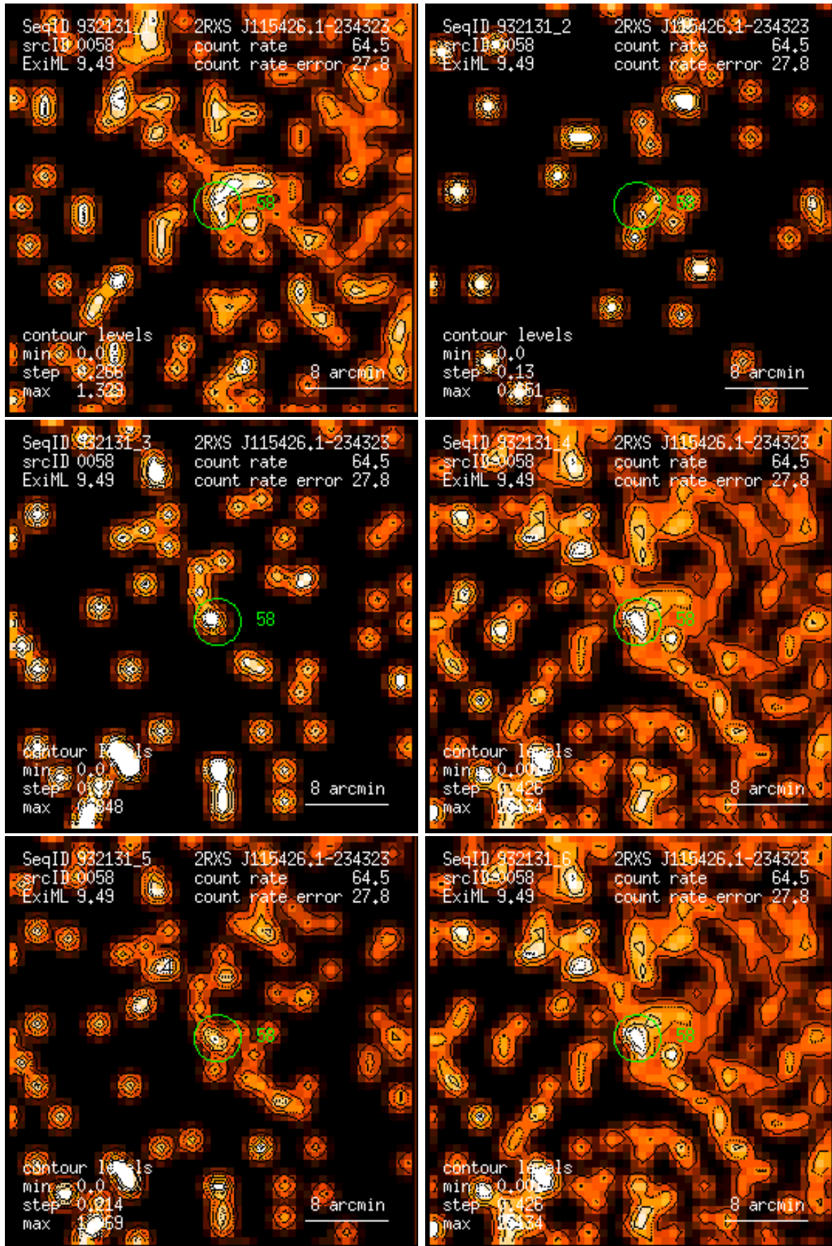
Figure 58: RASS 932131: detection 0058: band rate images, Gaussian filter: (1) PSPC channels 11 – 41, (2) 52 – 90, (3) 91 – 201, (4) 11 – 235, (5) 52 – 201, (6) 11 – 201. Broad band rates in counts/ks. Band rate contour levels in counts/ks/arcmin 2 .
