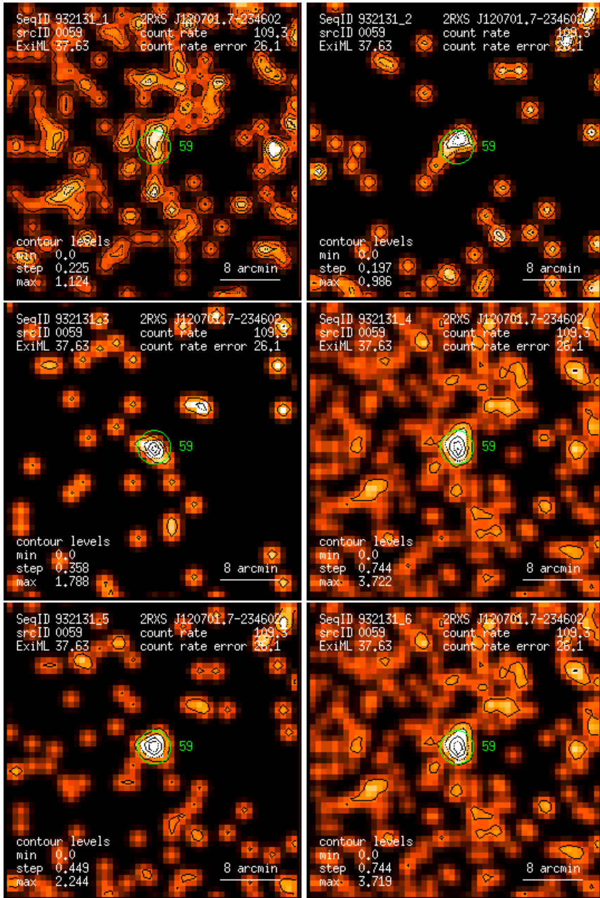
Figure 59: RASS 932131: detection 0059: band rate images, Gaussian filter: (1) PSPC channels 11 – 41, (2) 52 – 90, (3) 91 – 201, (4) 11 – 235, (5) 52 – 201, (6) 11 – 201. Broad band rates in counts/ks. Band rate contour levels in counts/ks/arcmin 2 .
