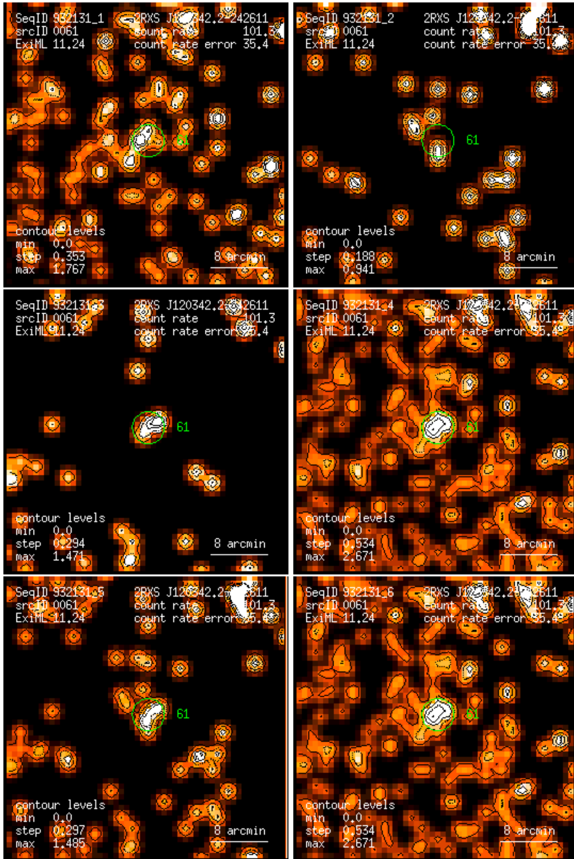
Figure 61: RASS 932131: detection 0061: band rate images, Gaussian filter: (1) PSPC channels 11 – 41, (2) 52 – 90, (3) 91 – 201, (4) 11 – 235, (5) 52 – 201, (6) 11 – 201. Broad band rates in counts/ks. Band rate contour levels in counts/ks/arcmin 2 .
