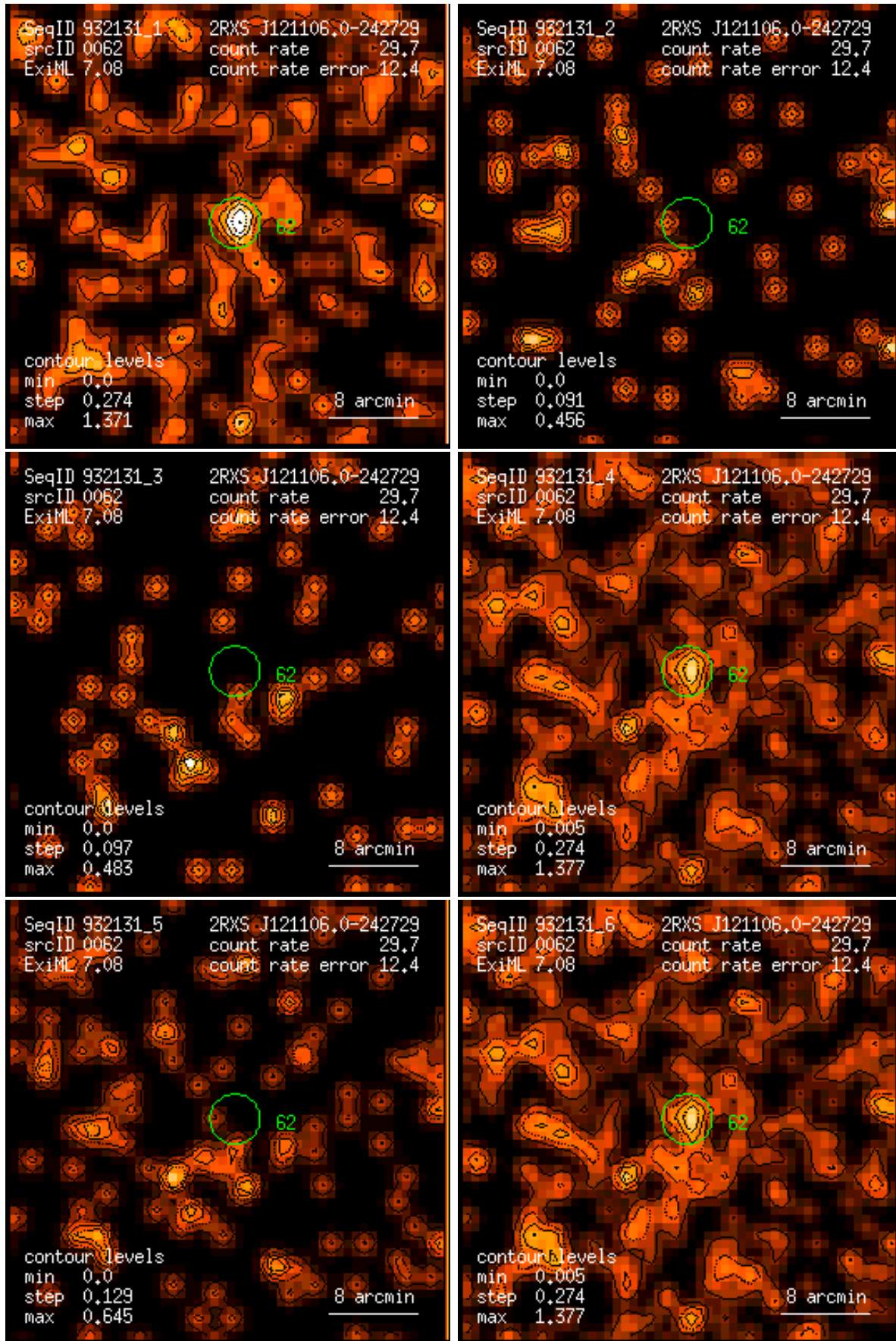
Figure 62: RASS 932131: detection 0062: band rate images, Gaussian filter: (1) PSPC channels 11 – 41, (2) 52 – 90, (3) 91 – 201, (4) 11 – 235, (5) 52 – 201, (6) 11 – 201. Broad band rates in counts/ks. Band rate contour levels in counts/ks/arcmin 2 .
