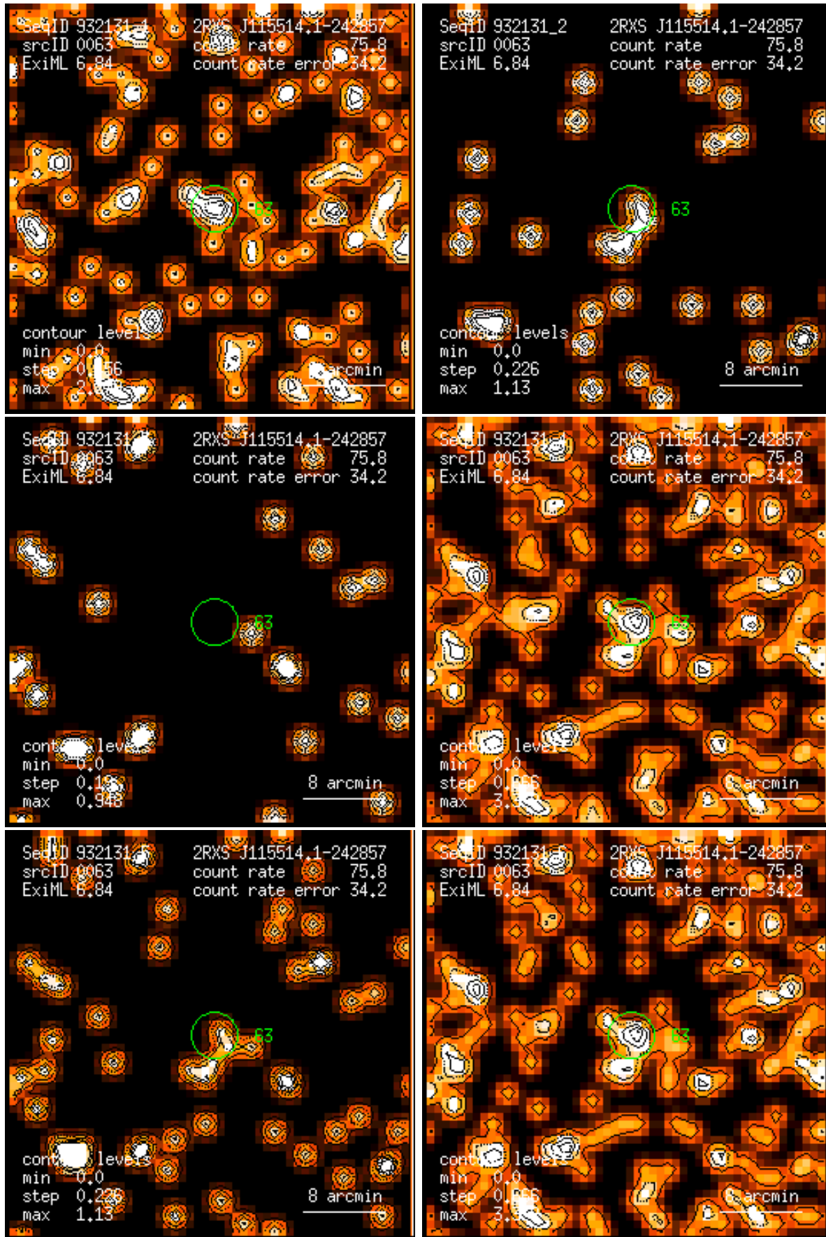
Figure 63: RASS 932131: detection 0063: band rate images, Gaussian filter: (1) PSPC channels 11 – 41, (2) 52 – 90, (3) 91 – 201, (4) 11 – 235, (5) 52 – 201, (6) 11 – 201. Broad band rates in counts/ks. Band rate contour levels in counts/ks/arcmin 2 .
