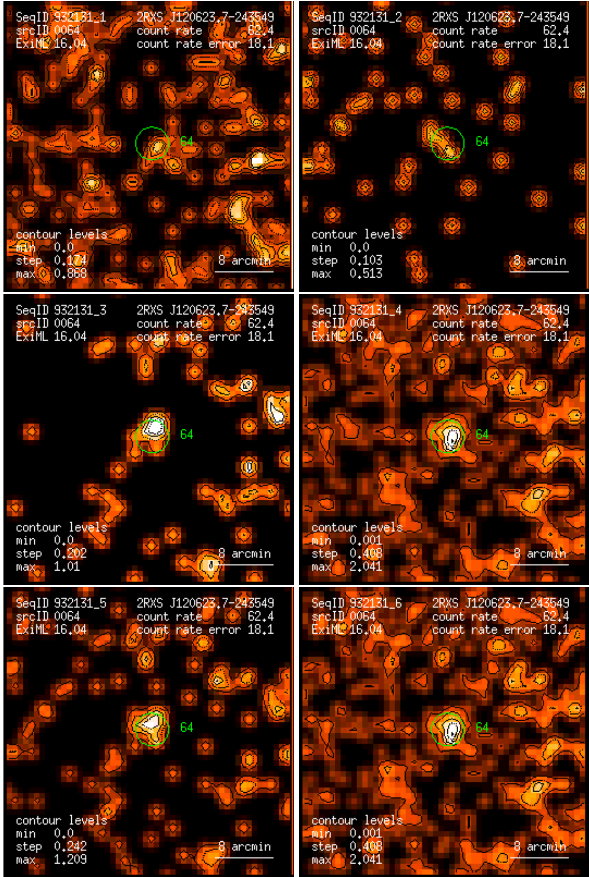
Figure 64: RASS 932131: detection 0064: band rate images, Gaussian filter: (1) PSPC channels 11 – 41, (2) 52 – 90, (3) 91 – 201, (4) 11 – 235, (5) 52 – 201, (6) 11 – 201. Broad band rates in counts/ks. Band rate contour levels in counts/ks/arcmin 2 .
