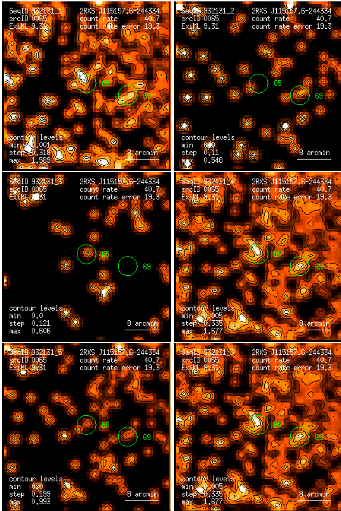
Figure 65: RASS 932131: detection 0065: band rate images, Gaussian filter: (1) PSPC channels 11 – 41, (2) 52 – 90, (3) 91 – 201, (4) 11 – 235, (5) 52 – 201, (6) 11 – 201. Broad band rates in counts/ks. Band rate contour levels in counts/ks/arcmin 2 .
