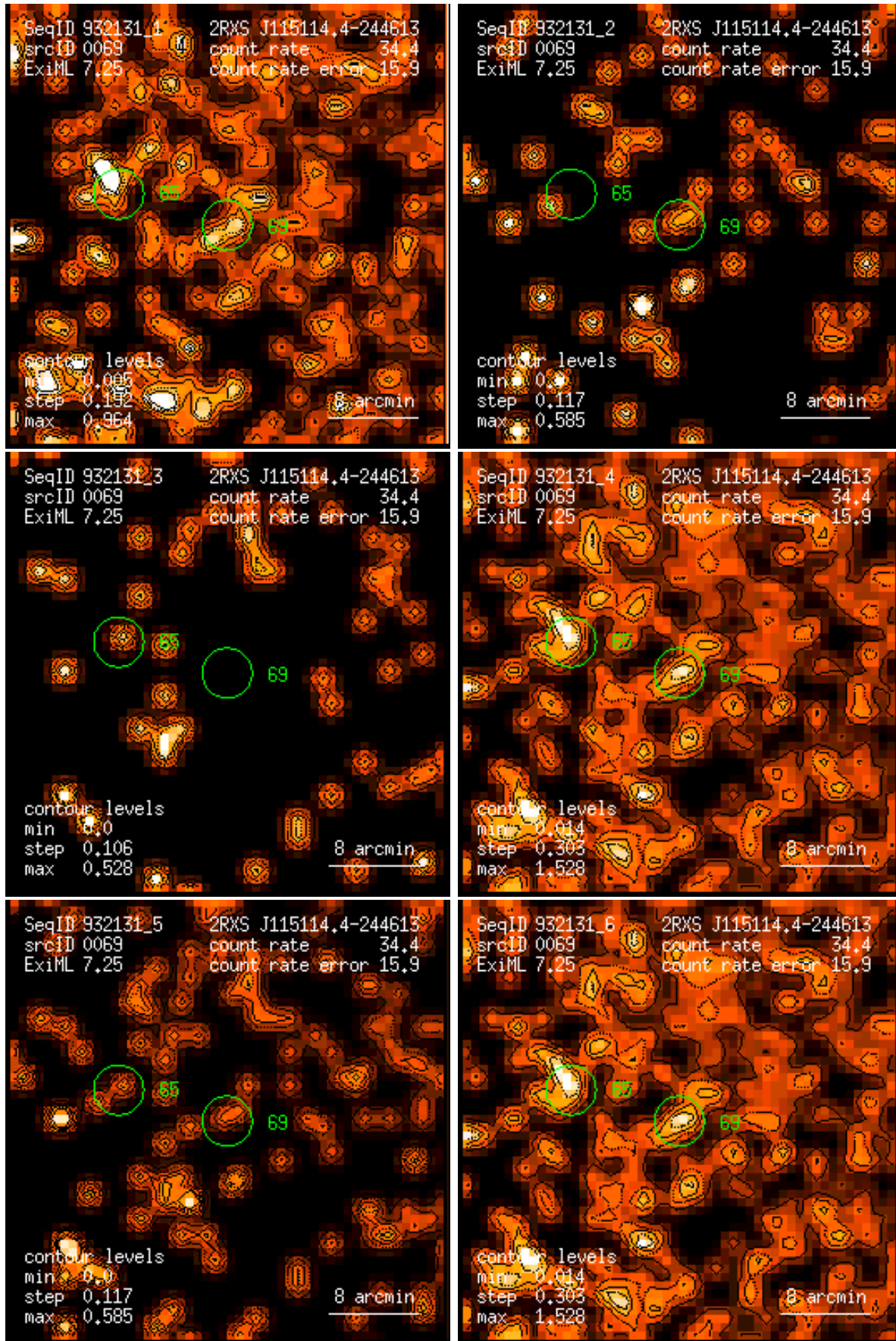
Figure 69: RASS 932131: detection 0069: band rate images, Gaussian filter: (1) PSPC channels 11 – 41, (2) 52 – 90, (3) 91 – 201, (4) 11 – 235, (5) 52 – 201, (6) 11 – 201. Broad band rates in counts/ks. Band rate contour levels in counts/ks/arcmin 2 .
