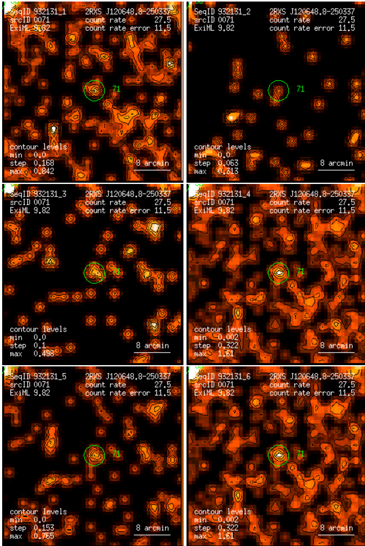
Figure 71: RASS 932131: detection 0071: band rate images, Gaussian filter: (1) PSPC channels 11 – 41, (2) 52 – 90, (3) 91 – 201, (4) 11 – 235, (5) 52 – 201, (6) 11 – 201. Broad band rates in counts/ks. Band rate contour levels in counts/ks/arcmin 2 .
