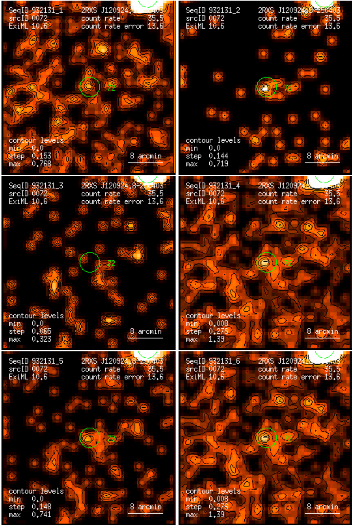
Figure 72: RASS 932131: detection 0072: band rate images, Gaussian filter: (1) PSPC channels 11 – 41, (2) 52 – 90, (3) 91 – 201, (4) 11 – 235, (5) 52 – 201, (6) 11 – 201. Broad band rates in counts/ks. Band rate contour levels in counts/ks/arcmin 2 .
