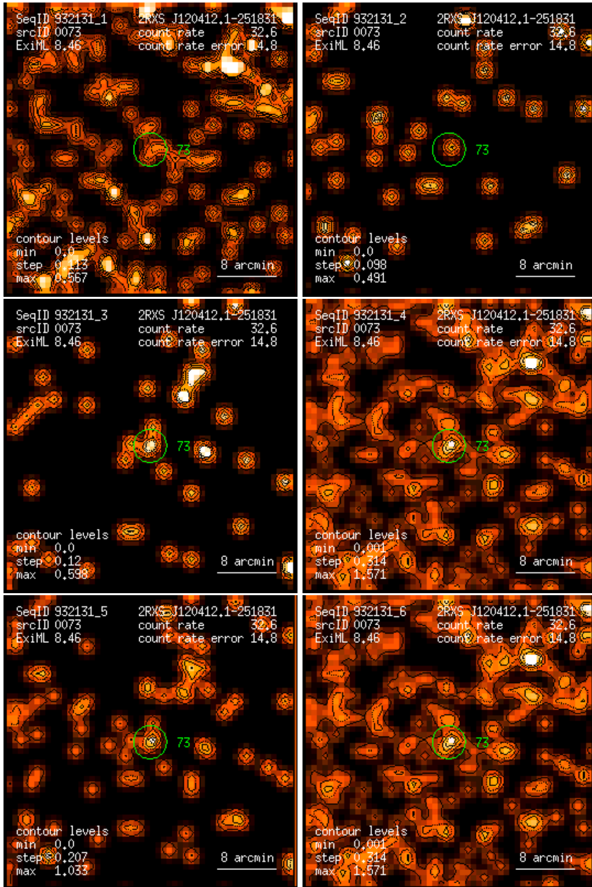
Figure 73: RASS 932131: detection 0073: band rate images, Gaussian filter: (1) PSPC channels 11 – 41, (2) 52 – 90, (3) 91 – 201, (4) 11 – 235, (5) 52 – 201, (6) 11 – 201. Broad band rates in counts/ks. Band rate contour levels in counts/ks/arcmin 2 .
