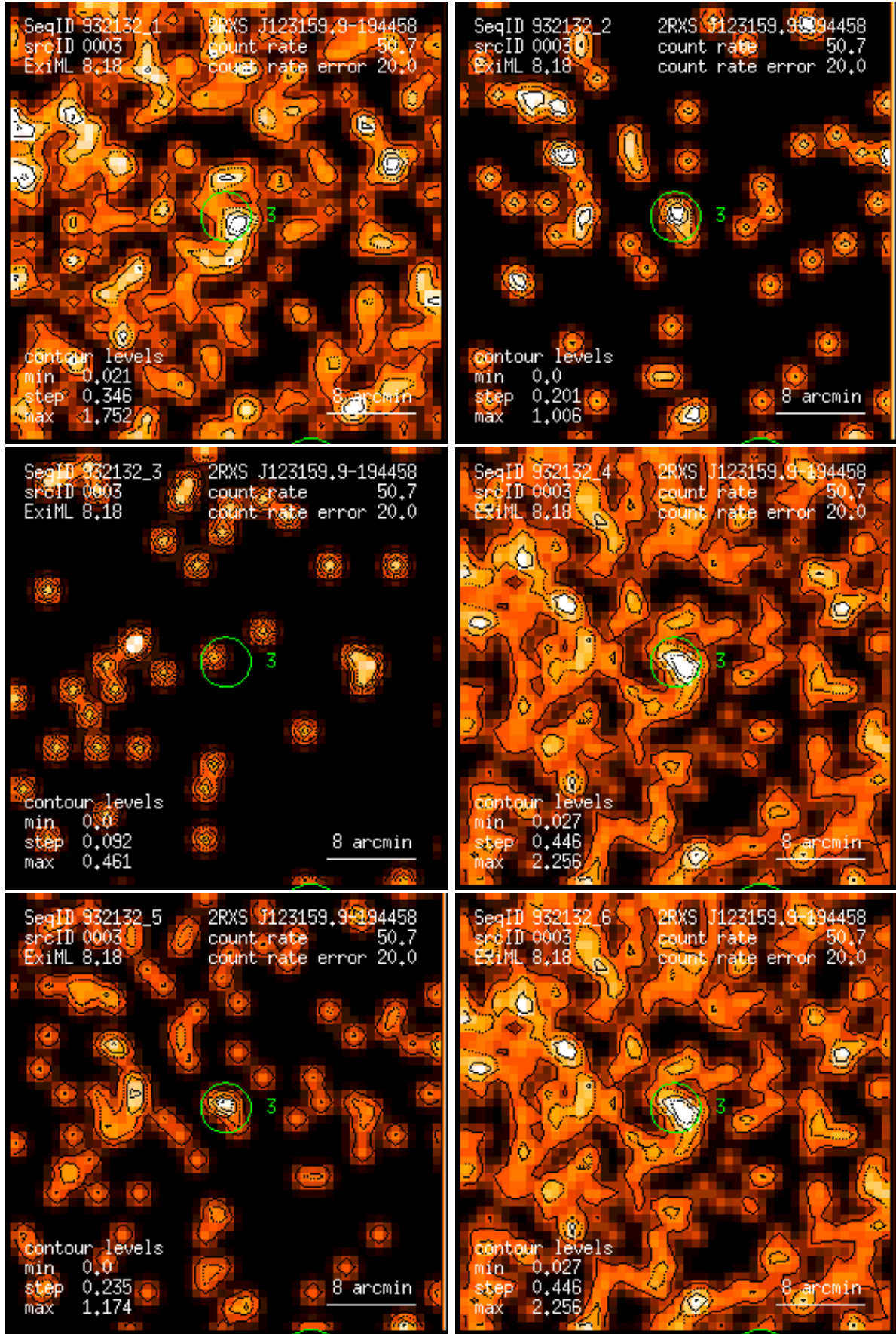
Figure 3: RASS 932132: detection 0003: band rate images, Gaussian filter: (1) PSPC channels 11 – 41, (2) 52 – 90, (3) 91 – 201, (4) 11 – 235, (5) 52 – 201, (6) 11 – 201. Broad band rates in counts/ks. Band rate contour levels in counts/ks/arcmin 2 .
