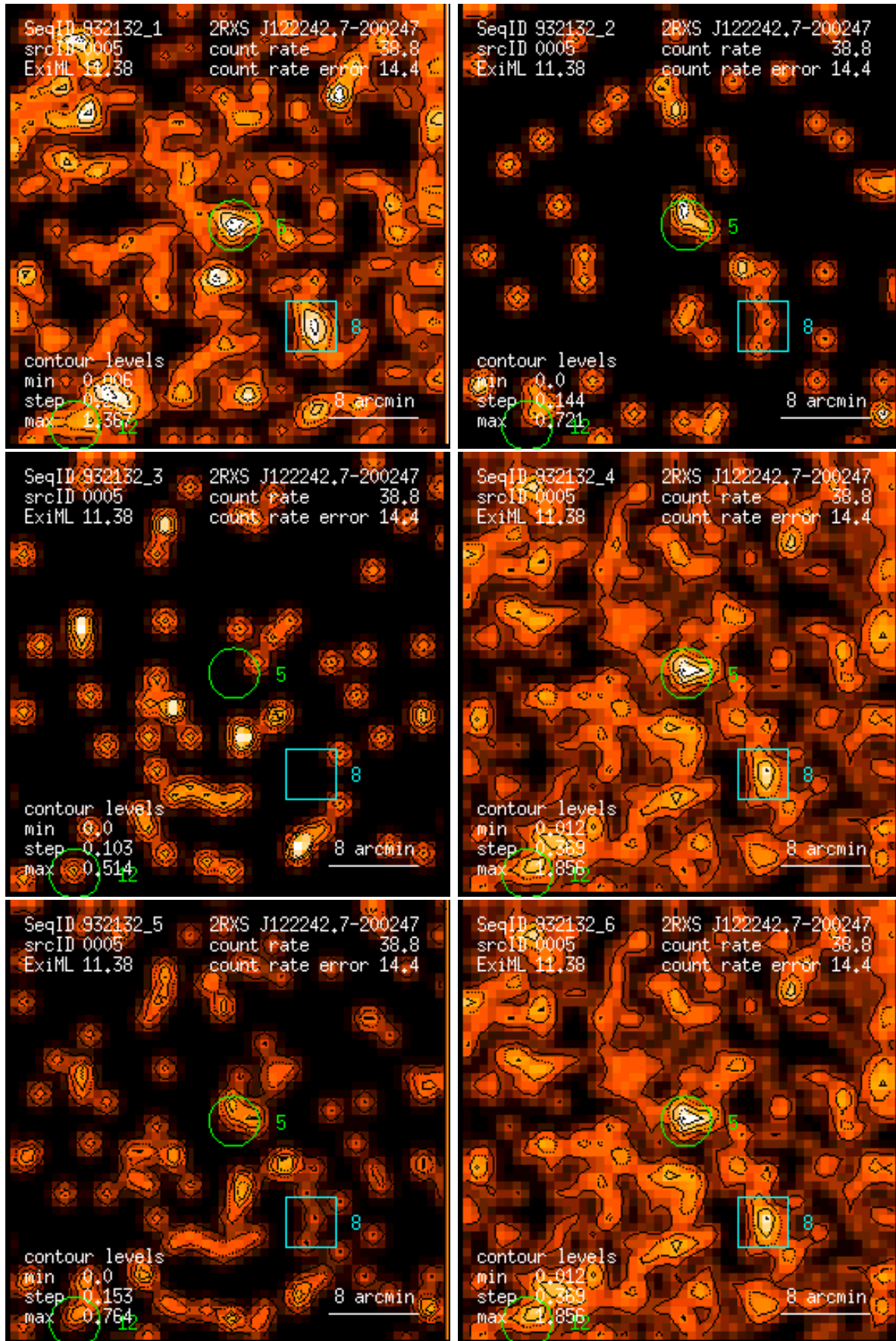
Figure 5: RASS 932132: detection 0005: band rate images, Gaussian filter: (1) PSPC channels 11 – 41, (2) 52 – 90, (3) 91 – 201, (4) 11 – 235, (5) 52 – 201, (6) 11 – 201. Broad band rates in counts/ks. Band rate contour levels in counts/ks/arcmin 2 .
