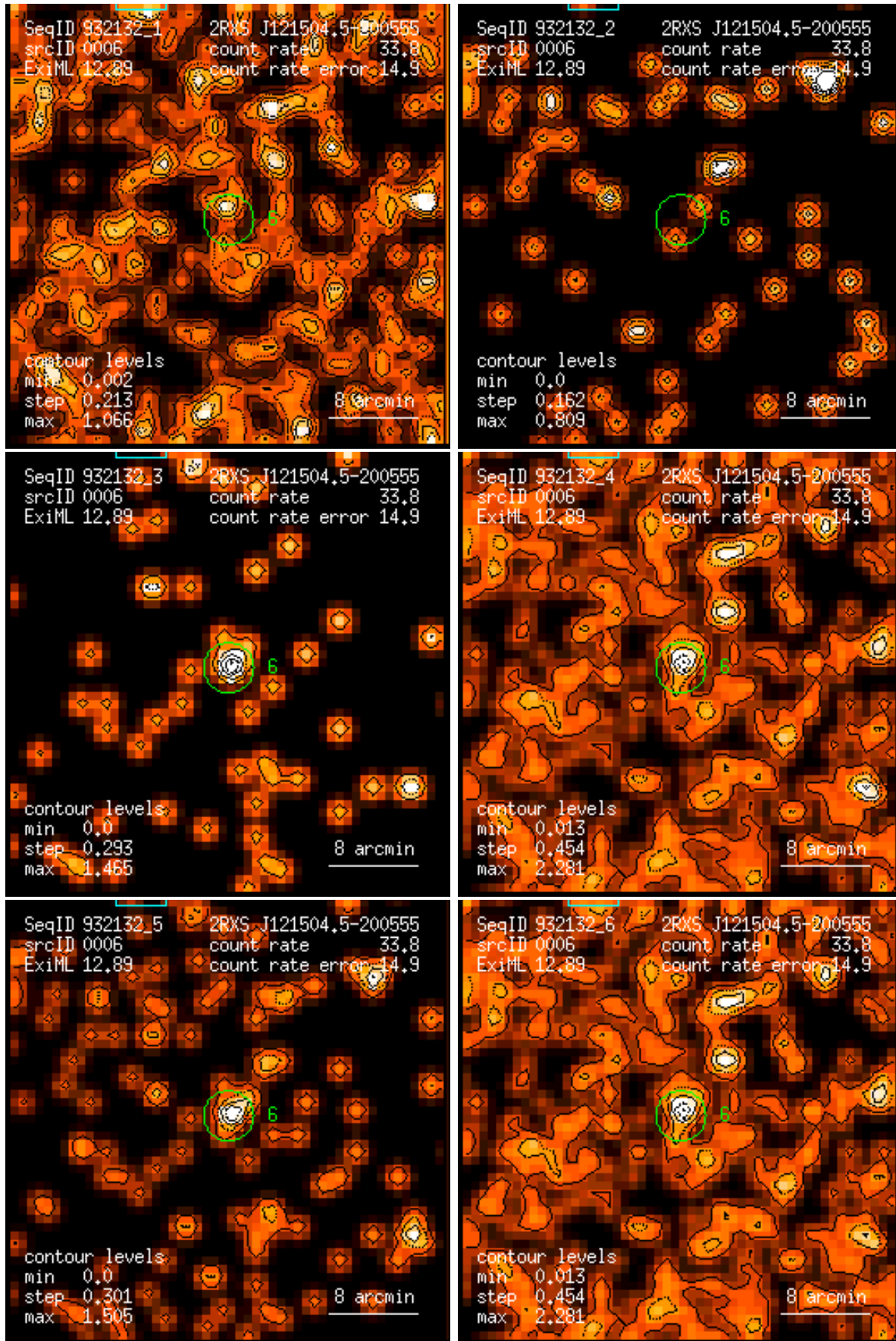
Figure 6: RASS 932132: detection 0006: band rate images, Gaussian filter: (1) PSPC channels 11 – 41, (2) 52 – 90, (3) 91 – 201, (4) 11 – 235, (5) 52 – 201, (6) 11 – 201. Broad band rates in counts/ks. Band rate contour levels in counts/ks/arcmin 2 .
