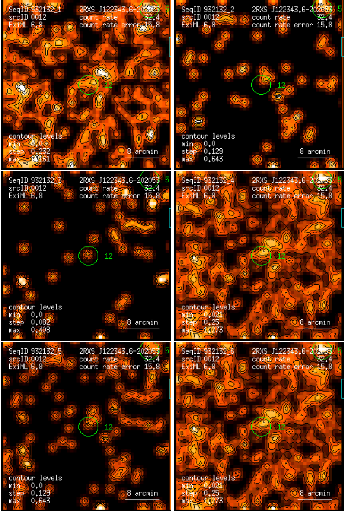
Figure 12: RASS 932132: detection 0012: band rate images, Gaussian filter: (1) PSPC channels 11 – 41, (2) 52 – 90, (3) 91 – 201, (4) 11 – 235, (5) 52 – 201, (6) 11 – 201. Broad band rates in counts/ks. Band rate contour levels in counts/ks/arcmin 2 .
