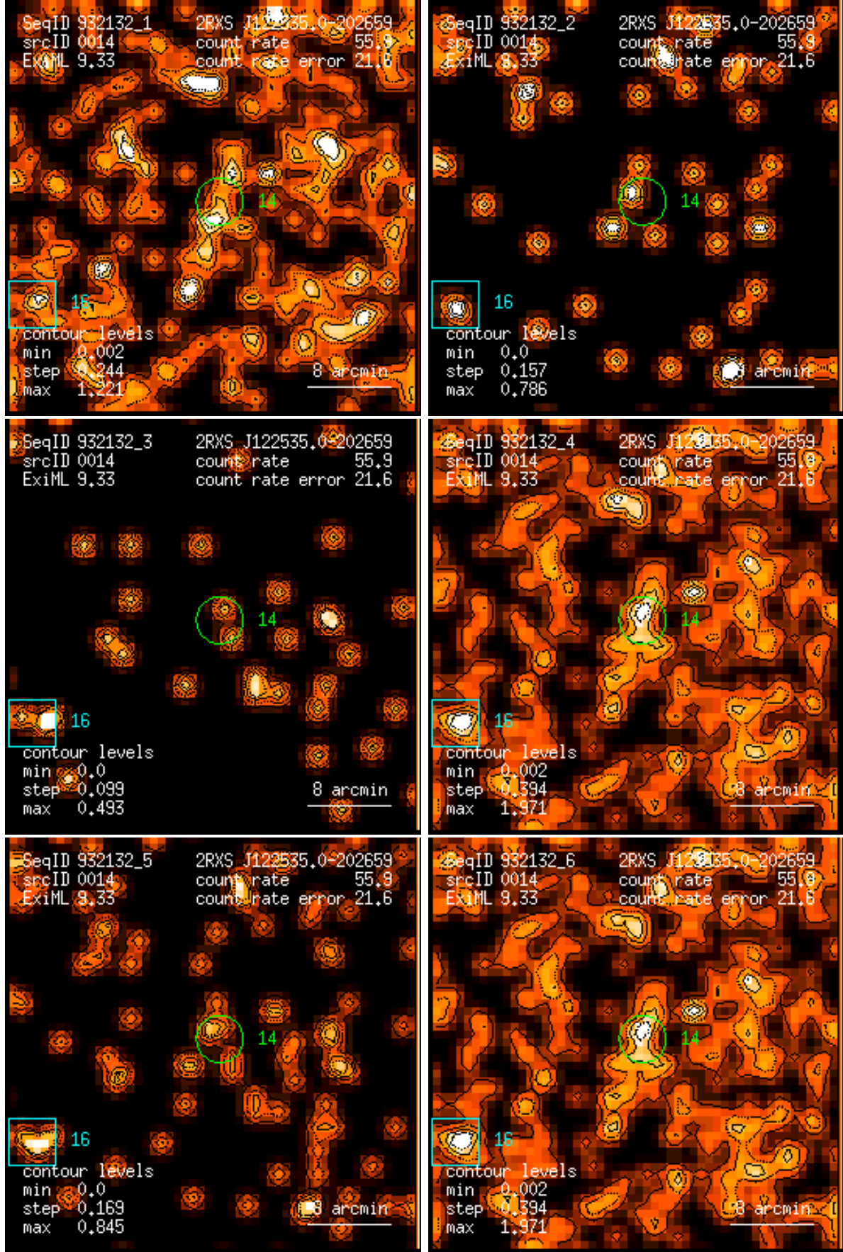
Figure 14: RASS 932132: detection 0014: band rate images, Gaussian filter: (1) PSPC channels 11 – 41, (2) 52 – 90, (3) 91 – 201, (4) 11 – 235, (5) 52 – 201, (6) 11 – 201. Broad band rates in counts/ks. Band rate contour levels in counts/ks/arcmin 2 .
