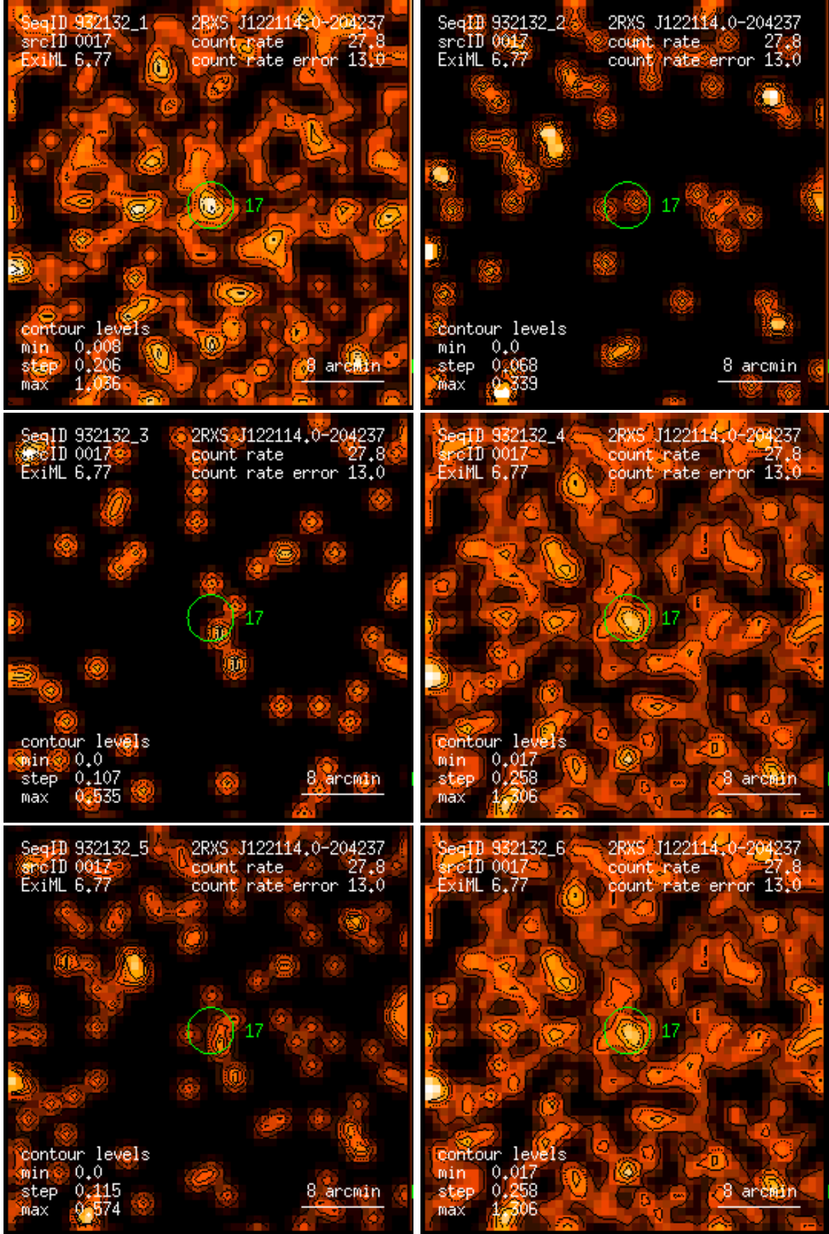
Figure 17: RASS 932132: detection 0017: band rate images, Gaussian filter: (1) PSPC channels 11 – 41, (2) 52 – 90, (3) 91 – 201, (4) 11 – 235, (5) 52 – 201, (6) 11 – 201. Broad band rates in counts/ks. Band rate contour levels in counts/ks/arcmin 2 .
