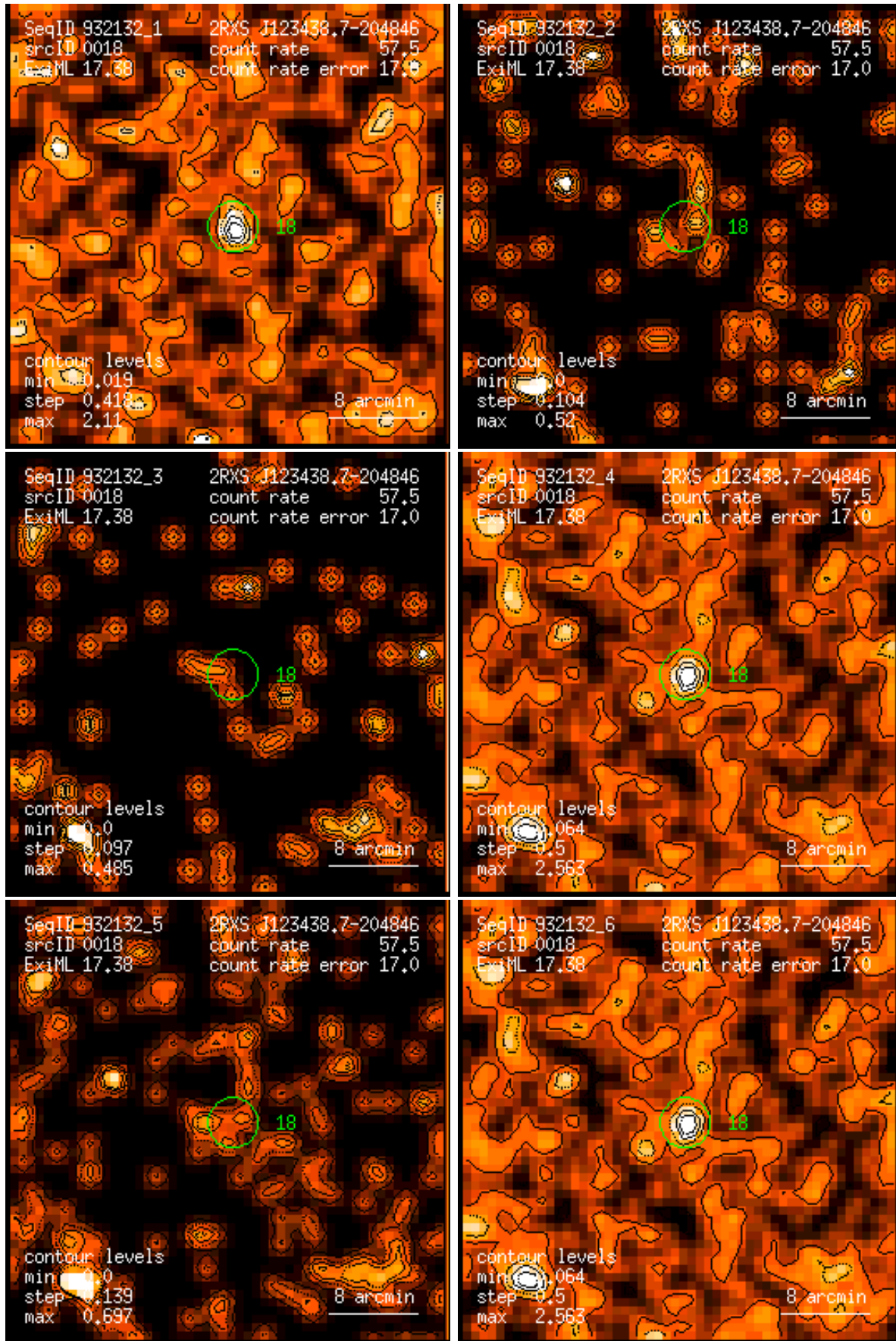
Figure 18: RASS 932132: detection 0018: band rate images, Gaussian filter: (1) PSPC channels 11 – 41, (2) 52 – 90, (3) 91 – 201, (4) 11 – 235, (5) 52 – 201, (6) 11 – 201. Broad band rates in counts/ks. Band rate contour levels in counts/ks/arcmin 2 .
