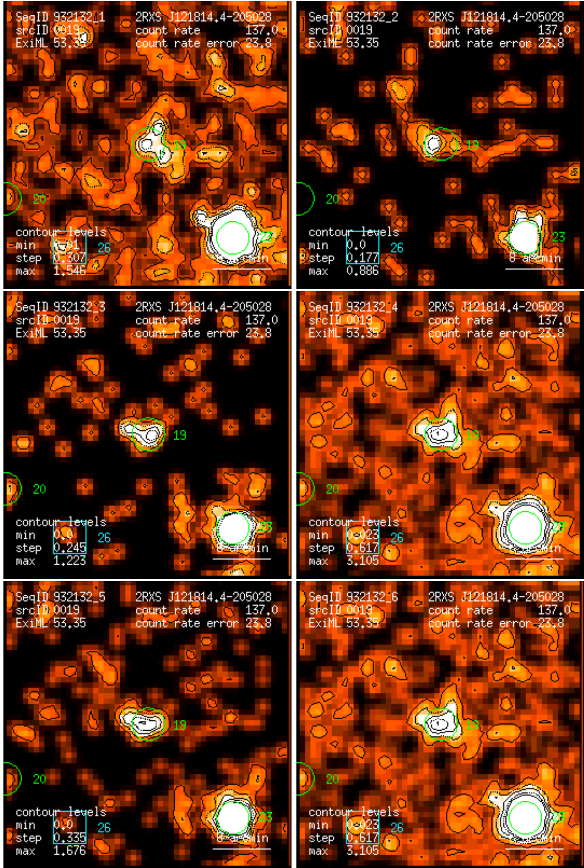
Figure 19: RASS 932132: detection 0019: band rate images, Gaussian filter: (1) PSPC channels 11 – 41, (2) 52 – 90, (3) 91 – 201, (4) 11 – 235, (5) 52 – 201, (6) 11 – 201. Broad band rates in counts/ks. Band rate contour levels in counts/ks/arcmin 2 .
