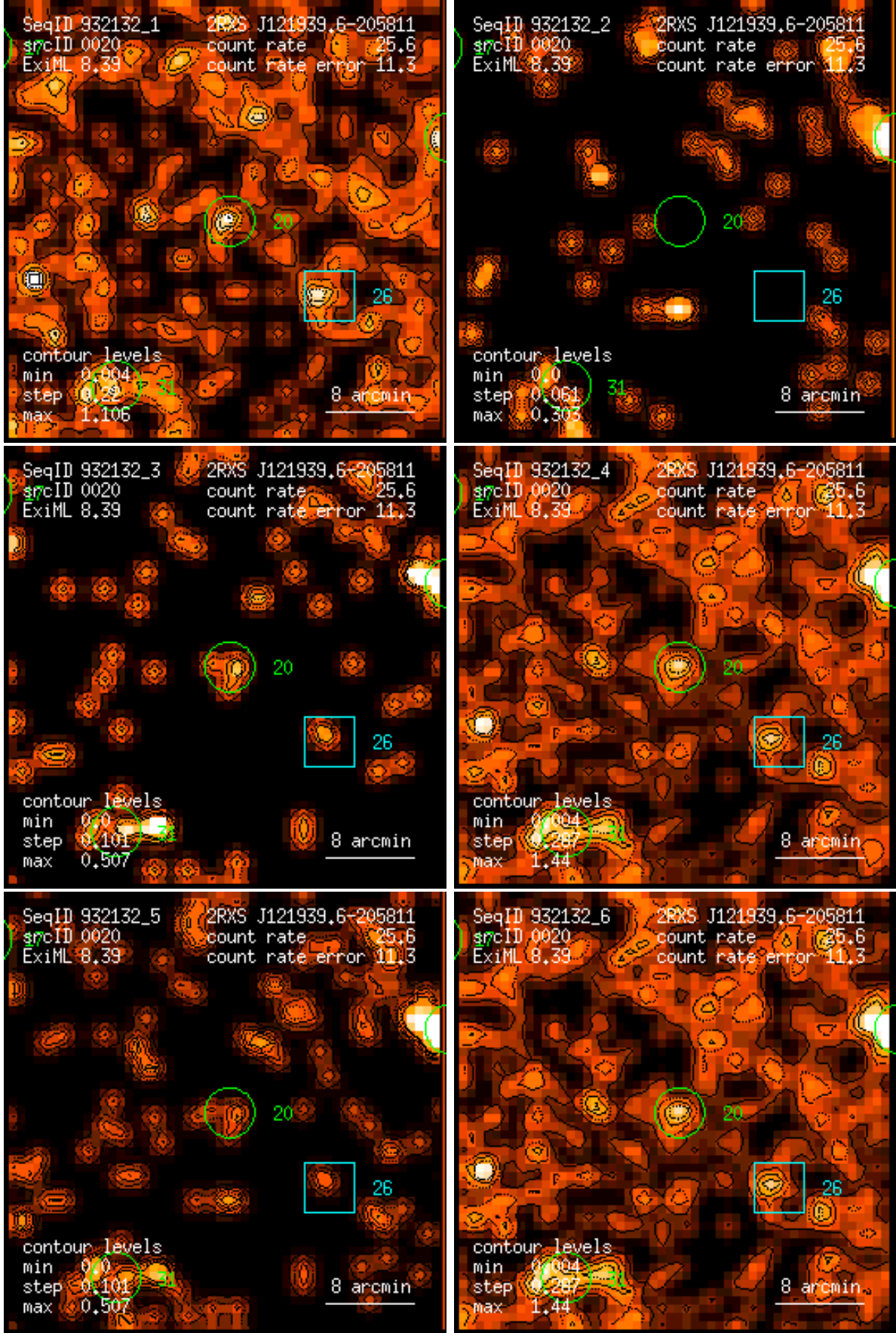
Figure 20: RASS 932132: detection 0020: band rate images, Gaussian filter: (1) PSPC channels 11 – 41, (2) 52 – 90, (3) 91 – 201, (4) 11 – 235, (5) 52 – 201, (6) 11 – 201. Broad band rates in counts/ks. Band rate contour levels in counts/ks/arcmin 2 .
