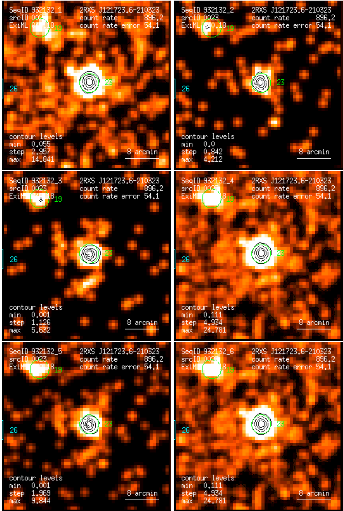
Figure 23: RASS 932132: detection 0023: band rate images, Gaussian filter: (1) PSPC channels 11 – 41, (2) 52 – 90, (3) 91 – 201, (4) 11 – 235, (5) 52 – 201, (6) 11 – 201. Broad band rates in counts/ks. Band rate contour levels in counts/ks/arcmin 2 .
