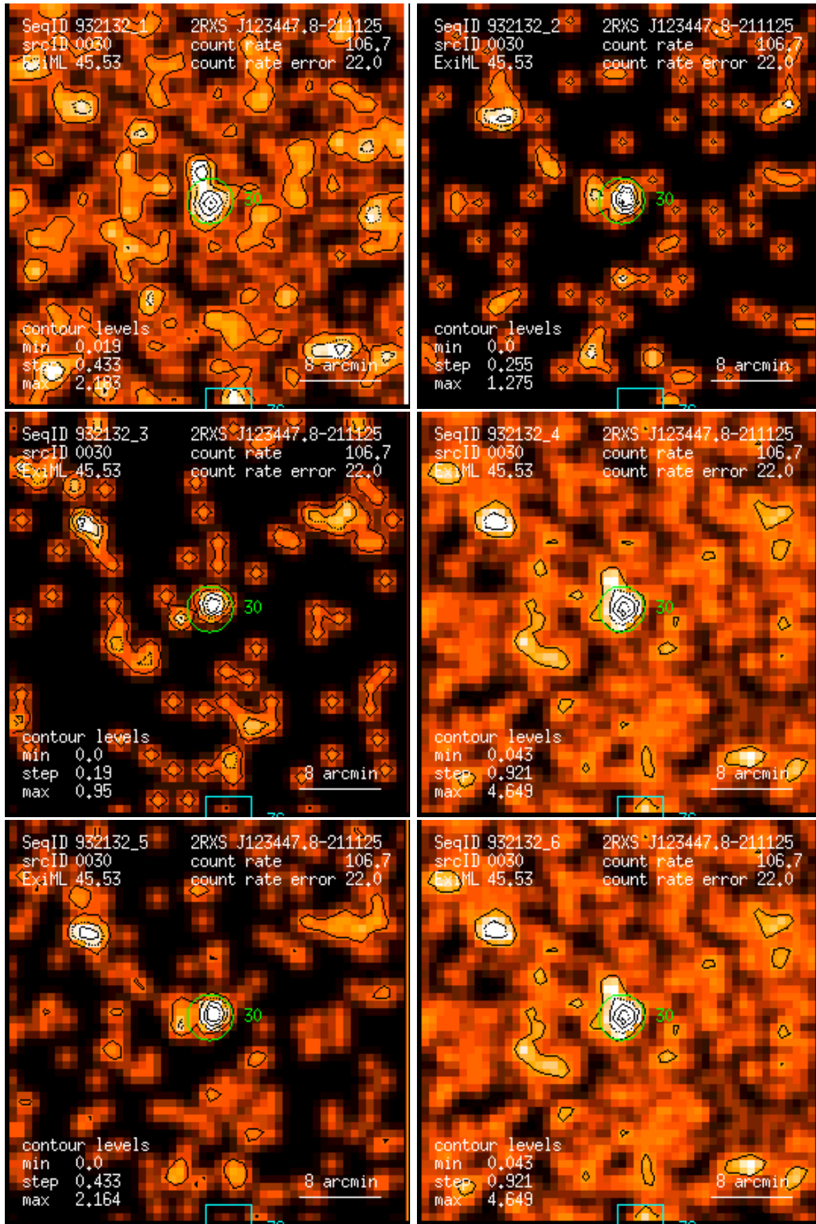
Figure 30: RASS 932132: detection 0030: band rate images, Gaussian filter: (1) PSPC channels 11 – 41, (2) 52 – 90, (3) 91 – 201, (4) 11 – 235, (5) 52 – 201, (6) 11 – 201. Broad band rates in counts/ks. Band rate contour levels in counts/ks/arcmin 2 .
