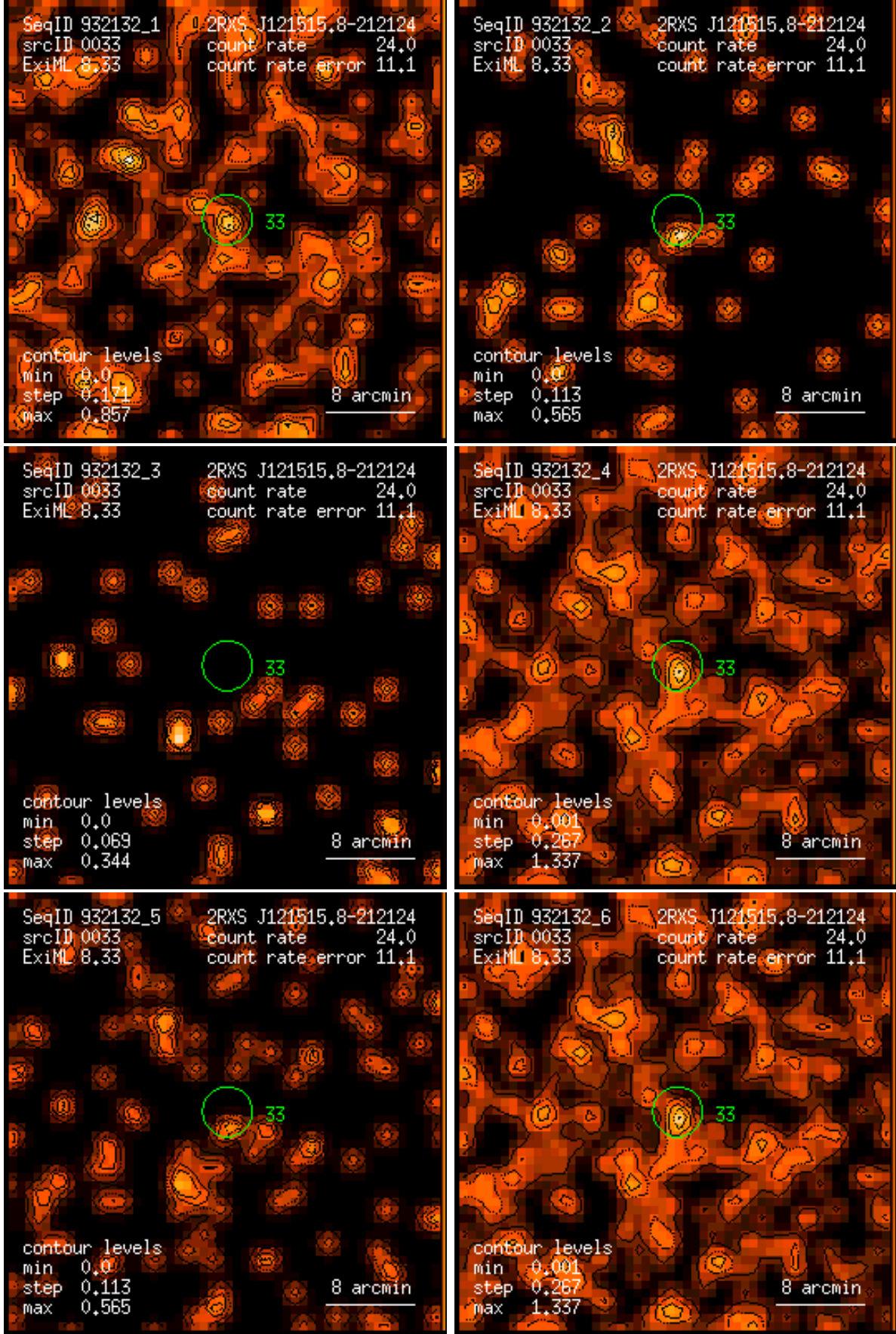
Figure 33: RASS 932132: detection 0033: band rate images, Gaussian filter: (1) PSPC channels 11 – 41, (2) 52 – 90, (3) 91 – 201, (4) 11 – 235, (5) 52 – 201, (6) 11 – 201. Broad band rates in counts/ks. Band rate contour levels in counts/ks/arcmin 2 .
