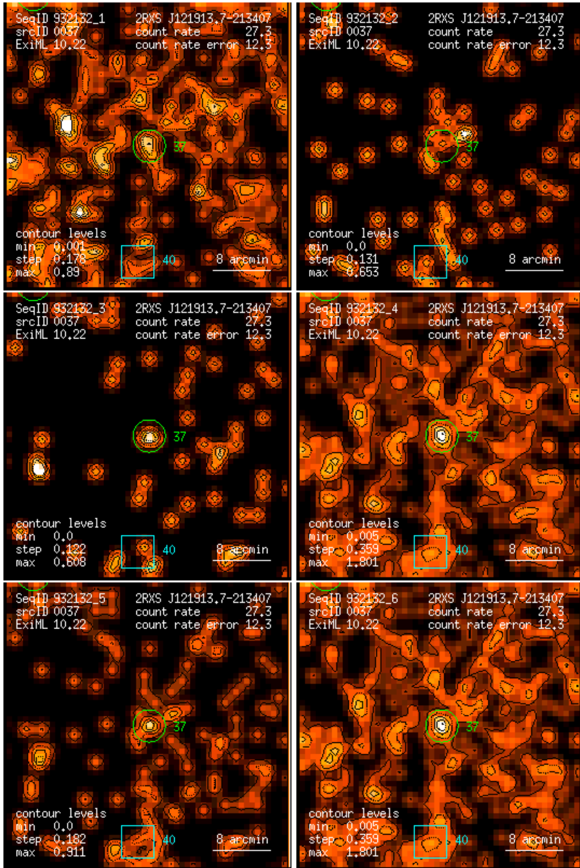
Figure 37: RASS 932132: detection 0037: band rate images, Gaussian filter: (1) PSPC channels 11 – 41, (2) 52 – 90, (3) 91 – 201, (4) 11 – 235, (5) 52 – 201, (6) 11 – 201. Broad band rates in counts/ks. Band rate contour levels in counts/ks/arcmin 2 .
