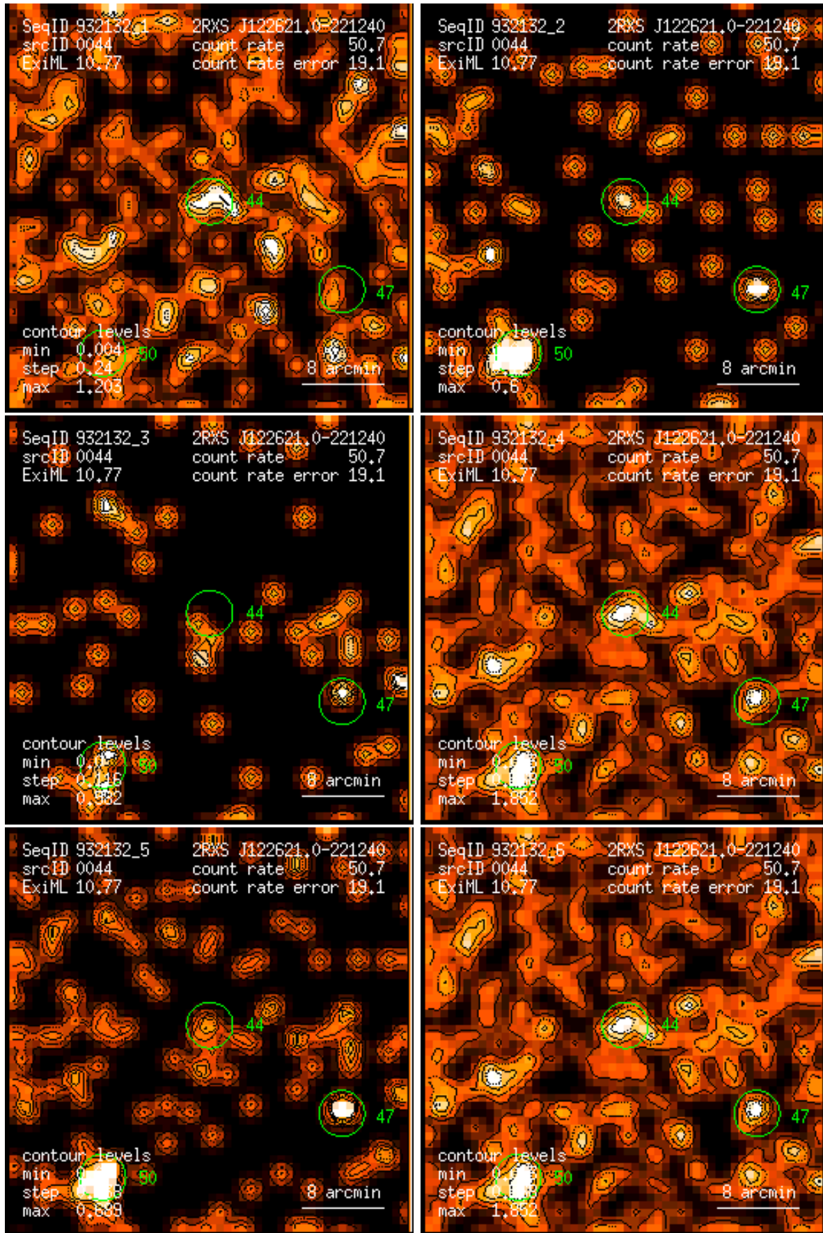
Figure 44: RASS 932132: detection 0044: band rate images, Gaussian filter: (1) PSPC channels 11 – 41, (2) 52 – 90, (3) 91 – 201, (4) 11 – 235, (5) 52 – 201, (6) 11 – 201. Broad band rates in counts/ks. Band rate contour levels in counts/ks/arcmin 2 .
