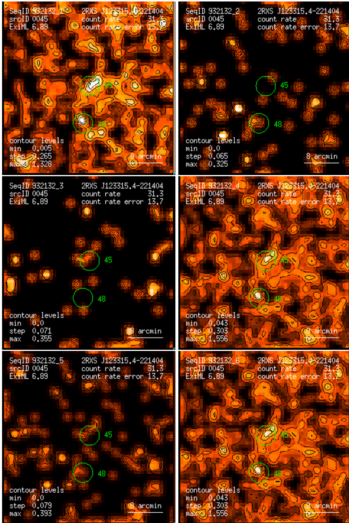
Figure 45: RASS 932132: detection 0045: band rate images, Gaussian filter: (1) PSPC channels 11 – 41, (2) 52 – 90, (3) 91 – 201, (4) 11 – 235, (5) 52 – 201, (6) 11 – 201. Broad band rates in counts/ks. Band rate contour levels in counts/ks/arcmin 2 .
