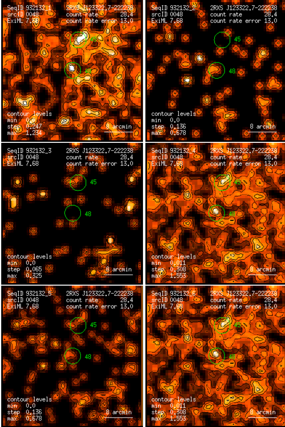
Figure 48: RASS 932132: detection 0048: band rate images, Gaussian filter: (1) PSPC channels 11 – 41, (2) 52 – 90, (3) 91 – 201, (4) 11 – 235, (5) 52 – 201, (6) 11 – 201. Broad band rates in counts/ks. Band rate contour levels in counts/ks/arcmin 2 .
