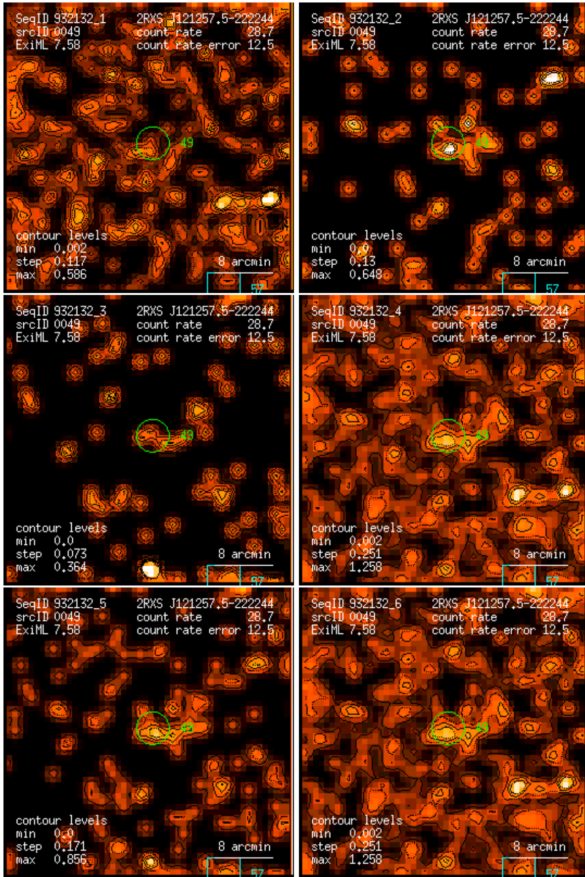
Figure 49: RASS 932132: detection 0049: band rate images, Gaussian filter: (1) PSPC channels 11 – 41, (2) 52 – 90, (3) 91 – 201, (4) 11 – 235, (5) 52 – 201, (6) 11 – 201. Broad band rates in counts/ks. Band rate contour levels in counts/ks/arcmin 2 .
