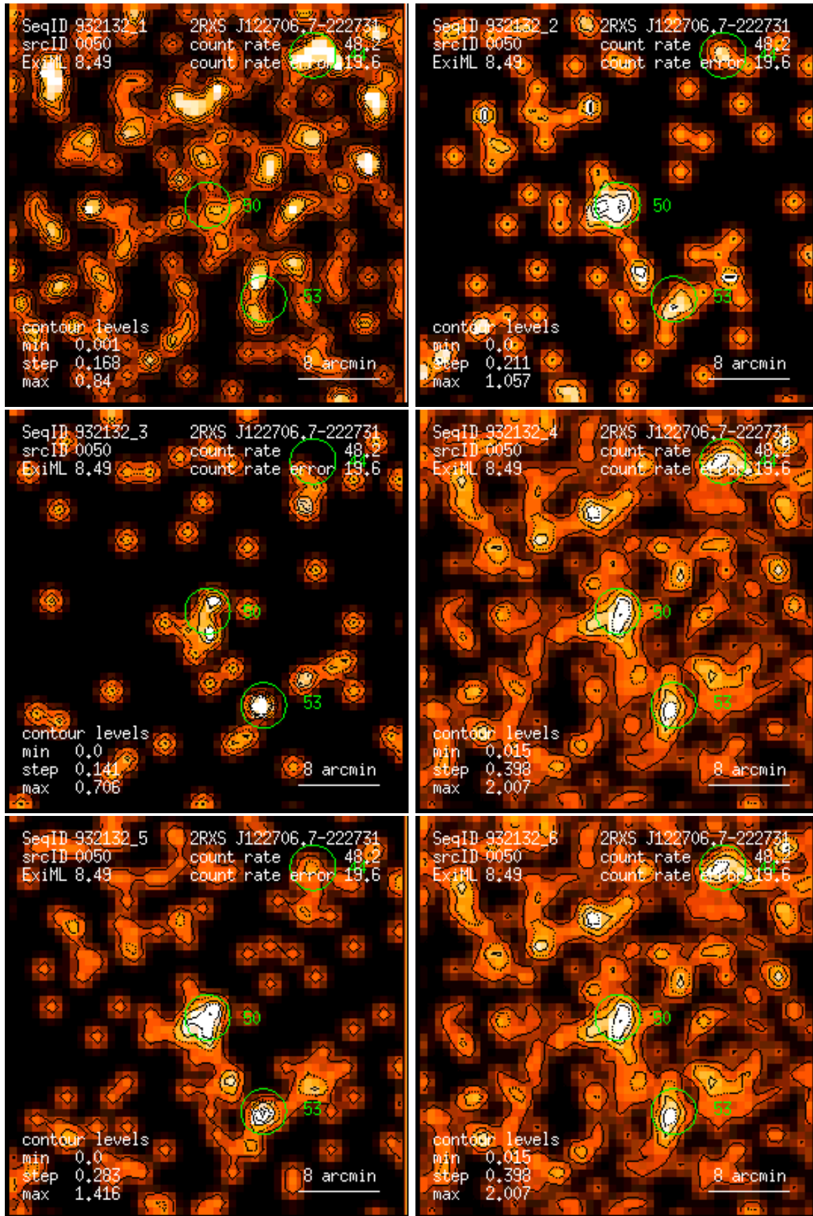
Figure 50: RASS 932132: detection 0050: band rate images, Gaussian filter: (1) PSPC channels 11 – 41, (2) 52 – 90, (3) 91 – 201, (4) 11 – 235, (5) 52 – 201, (6) 11 – 201. Broad band rates in counts/ks. Band rate contour levels in counts/ks/arcmin 2 .
