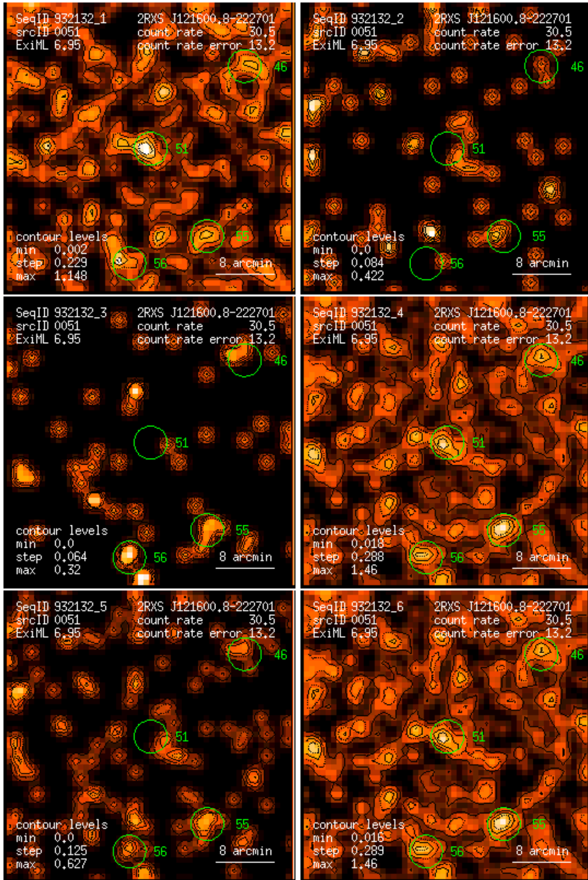
Figure 51: RASS 932132: detection 0051: band rate images, Gaussian filter: (1) PSPC channels 11 – 41, (2) 52 – 90, (3) 91 – 201, (4) 11 – 235, (5) 52 – 201, (6) 11 – 201. Broad band rates in counts/ks. Band rate contour levels in counts/ks/arcmin 2 .
