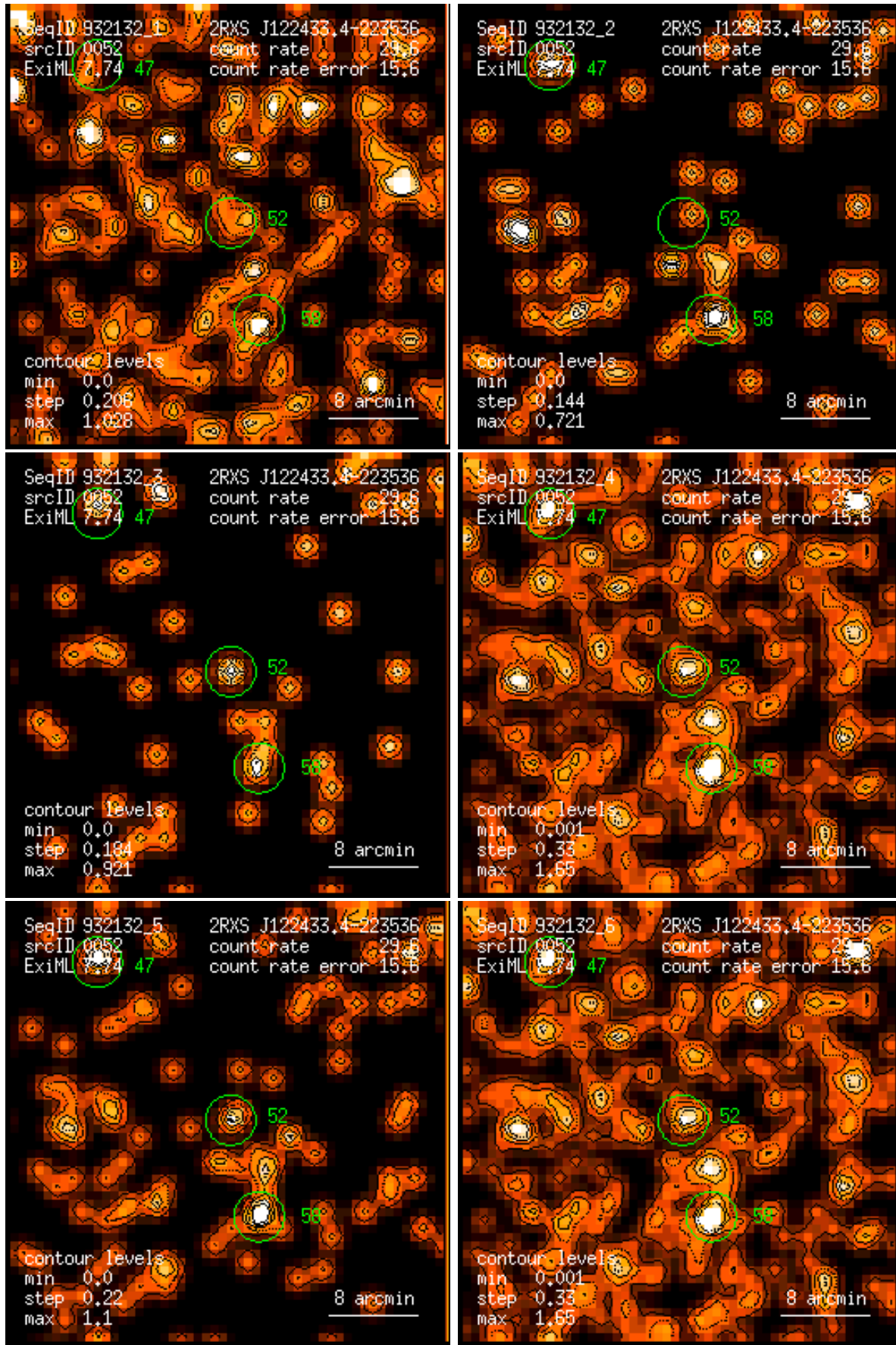
Figure 52: RASS 932132: detection 0052: band rate images, Gaussian filter: (1) PSPC channels 11 – 41, (2) 52 – 90, (3) 91 – 201, (4) 11 – 235, (5) 52 – 201, (6) 11 – 201. Broad band rates in counts/ks. Band rate contour levels in counts/ks/arcmin 2 .
