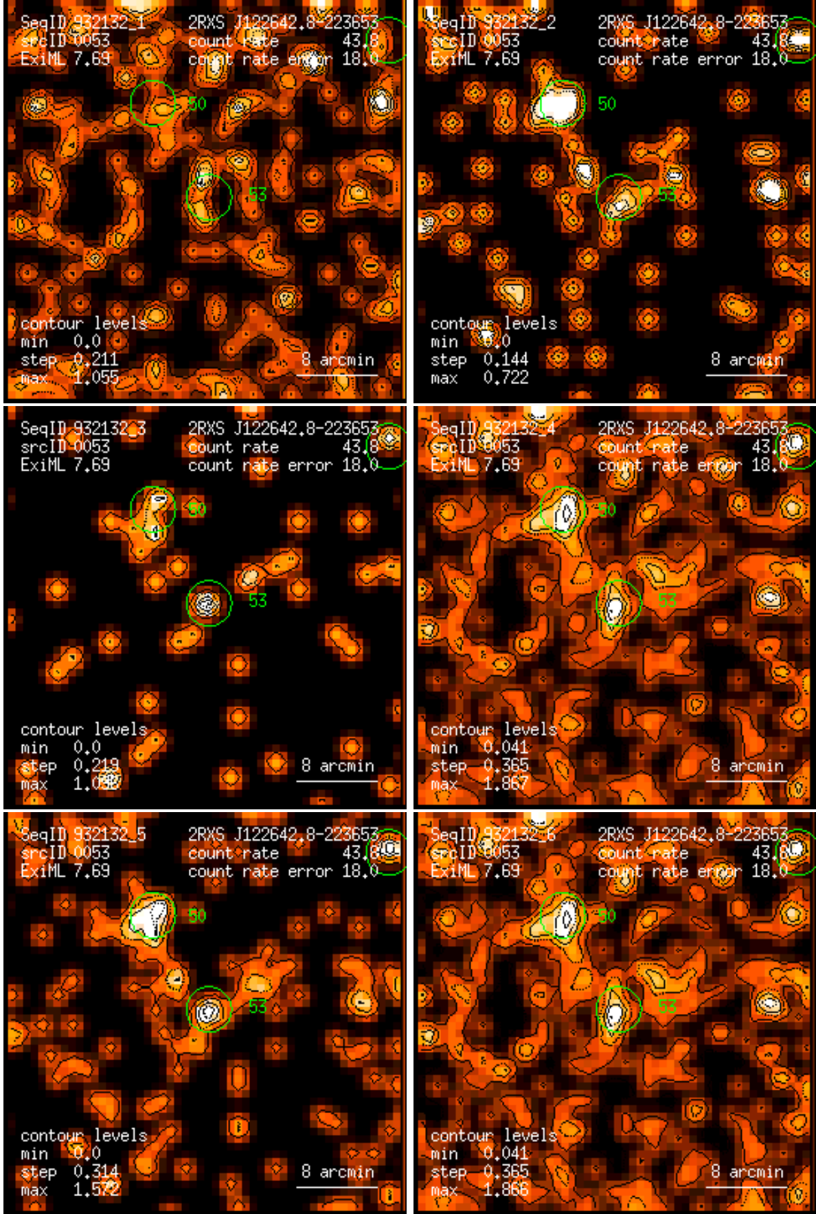
Figure 53: RASS 932132: detection 0053: band rate images, Gaussian filter: (1) PSPC channels 11 – 41, (2) 52 – 90, (3) 91 – 201, (4) 11 – 235, (5) 52 – 201, (6) 11 – 201. Broad band rates in counts/ks. Band rate contour levels in counts/ks/arcmin 2 .
