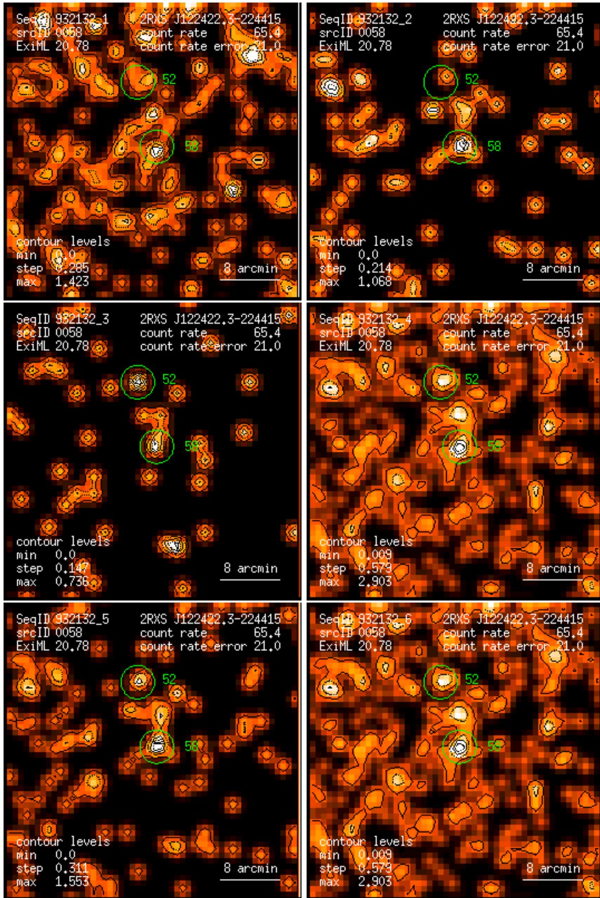
Figure 58: RASS 932132: detection 0058: band rate images, Gaussian filter: (1) PSPC channels 11 – 41, (2) 52 – 90, (3) 91 – 201, (4) 11 – 235, (5) 52 – 201, (6) 11 – 201. Broad band rates in counts/ks. Band rate contour levels in counts/ks/arcmin 2 .
