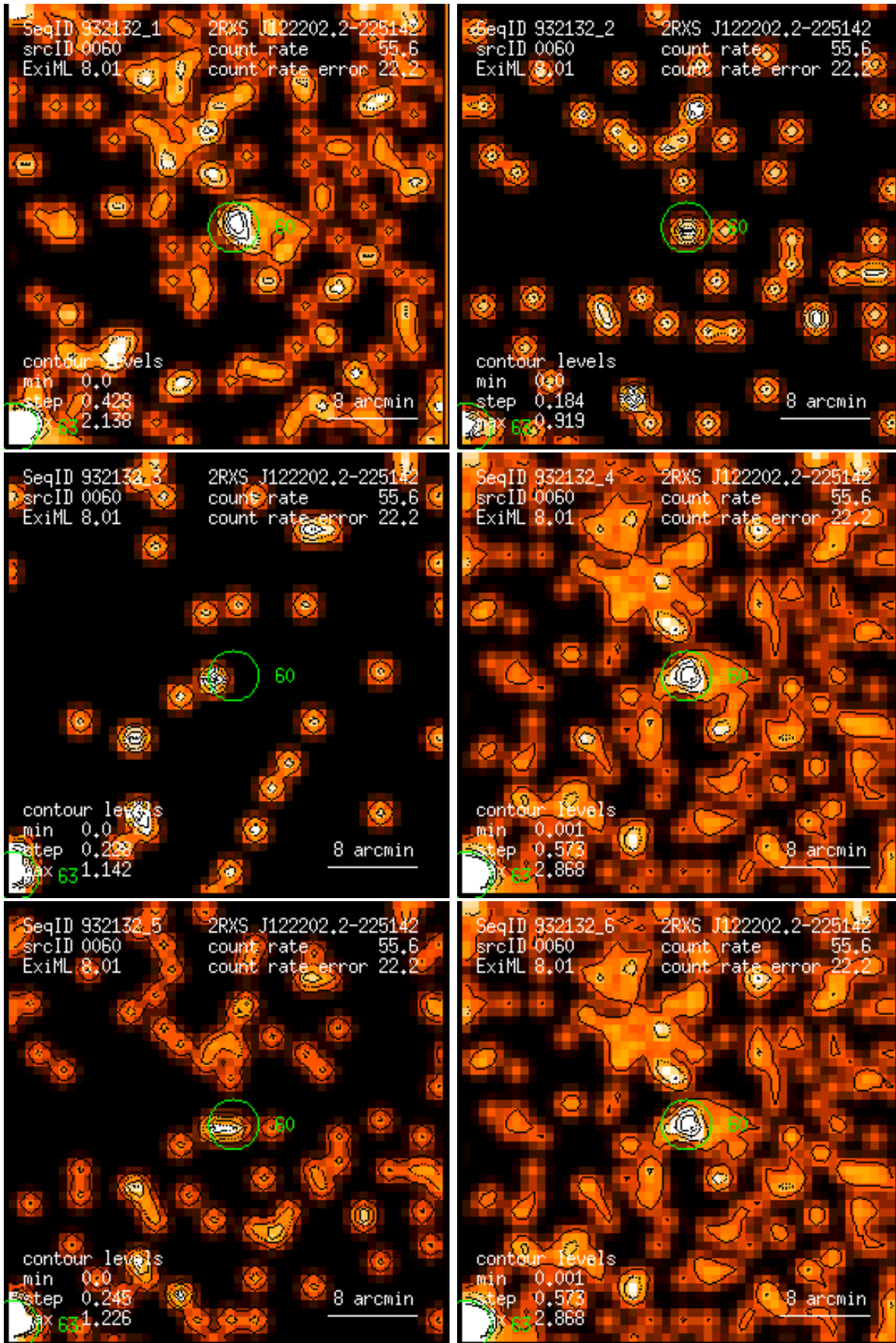
Figure 60: RASS 932132: detection 0060: band rate images, Gaussian filter: (1) PSPC channels 11 – 41, (2) 52 – 90, (3) 91 – 201, (4) 11 – 235, (5) 52 – 201, (6) 11 – 201. Broad band rates in counts/ks. Band rate contour levels in counts/ks/arcmin 2 .
