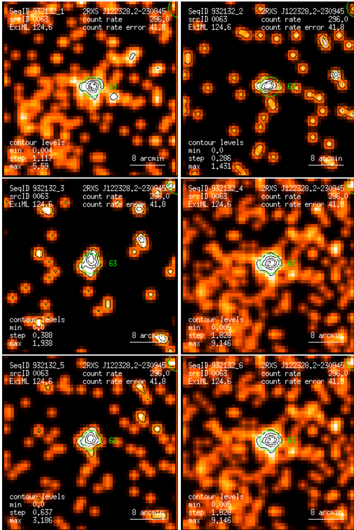
Figure 63: RASS 932132: detection 0063: band rate images, Gaussian filter: (1) PSPC channels 11 – 41, (2) 52 – 90, (3) 91 – 201, (4) 11 – 235, (5) 52 – 201, (6) 11 – 201. Broad band rates in counts/ks. Band rate contour levels in counts/ks/arcmin 2 .
