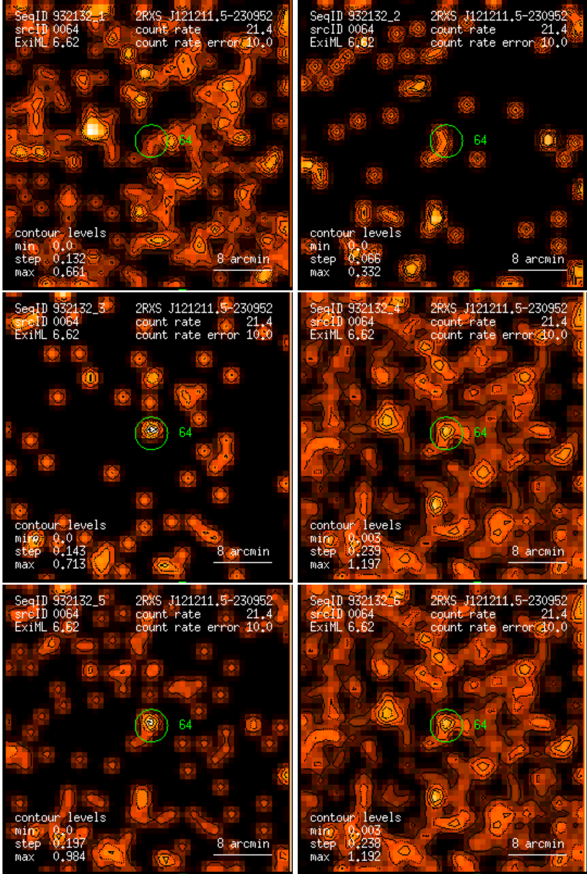
Figure 64: RASS 932132: detection 0064: band rate images, Gaussian filter: (1) PSPC channels 11 – 41, (2) 52 – 90, (3) 91 – 201, (4) 11 – 235, (5) 52 – 201, (6) 11 – 201. Broad band rates in counts/ks. Band rate contour levels in counts/ks/arcmin 2 .
