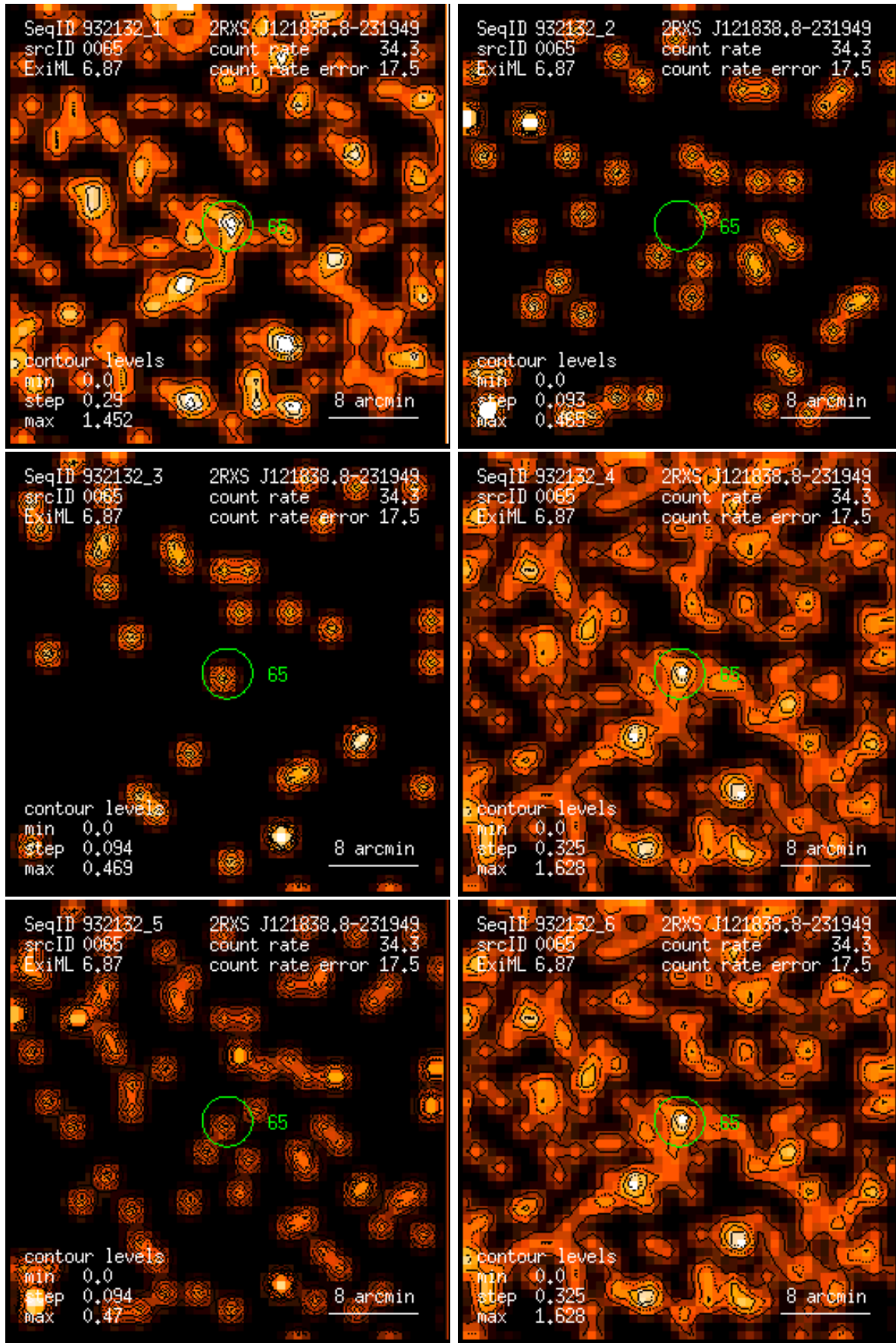
Figure 65: RASS 932132: detection 0065: band rate images, Gaussian filter: (1) PSPC channels 11 – 41, (2) 52 – 90, (3) 91 – 201, (4) 11 – 235, (5) 52 – 201, (6) 11 – 201. Broad band rates in counts/ks. Band rate contour levels in counts/ks/arcmin 2 .
