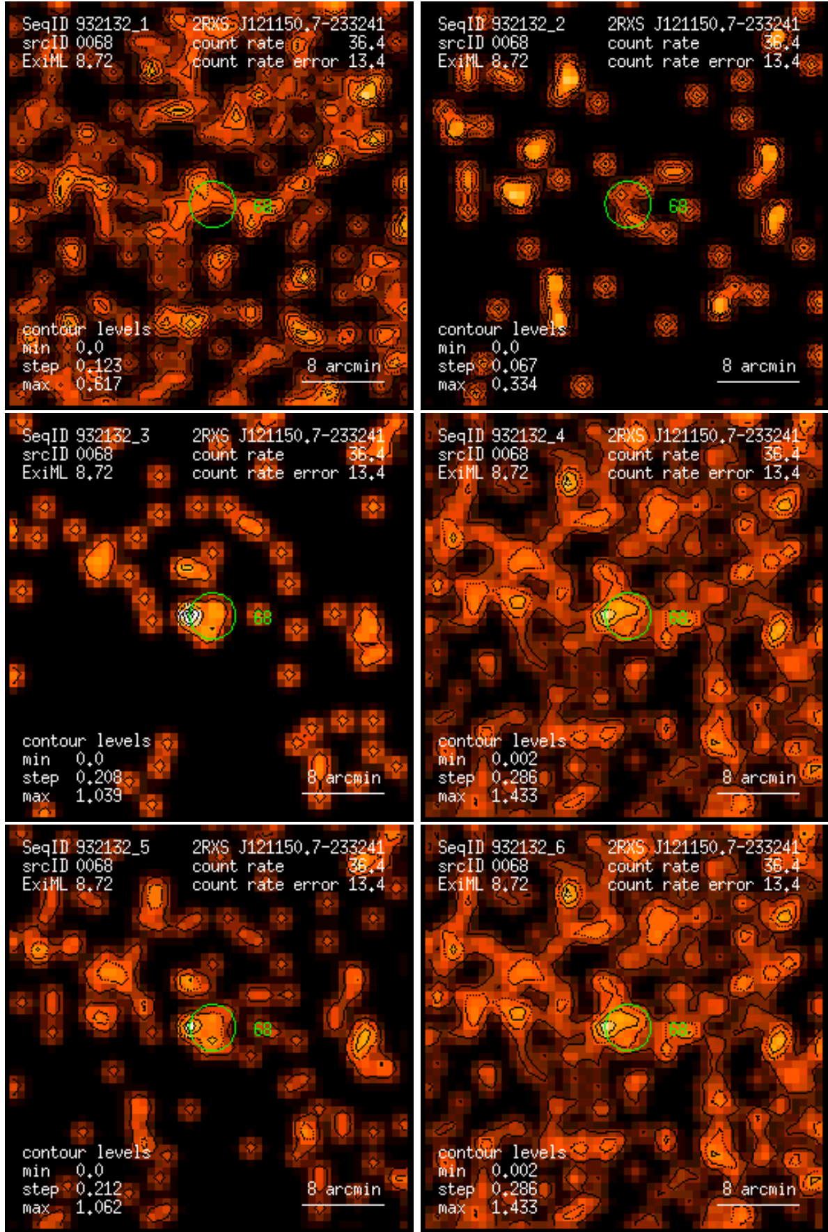
Figure 68: RASS 932132: detection 0068: band rate images, Gaussian filter: (1) PSPC channels 11 – 41, (2) 52 – 90, (3) 91 – 201, (4) 11 – 235, (5) 52 – 201, (6) 11 – 201. Broad band rates in counts/ks. Band rate contour levels in counts/ks/arcmin 2 .
